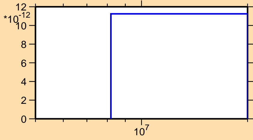
\sigma vs. E for ^{221}\text{At}(\text{mt } 45)
