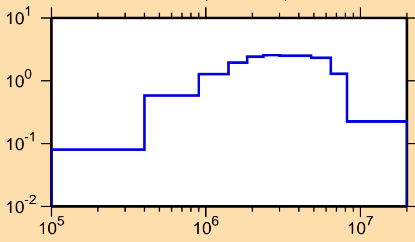
\sigma vs. E for ^{221}\text{At}(n,n\text{cont.})
