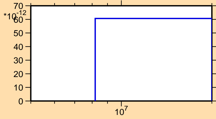
\sigma vs. E for ^{221}\text{At}(\text{mt117})
