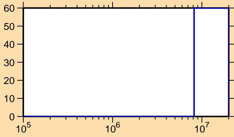
\Delta\sigma/\sigma vs. E for ^{221}\text{At}(n,f)
