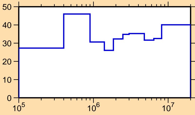
\Delta\sigma/\sigma vs. E for ^{221}\text{At}(n,\text{tot.})
