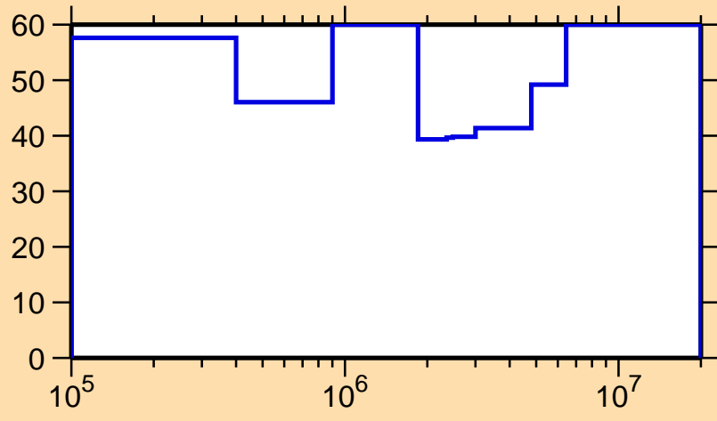
\Delta\sigma/\sigma vs. E for ^{221}\text{At}(n, el.)
