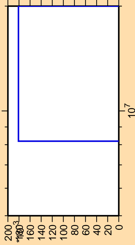
\Delta\sigma/\sigma vs. E for ^{221}\text{At}(\text{mt } 42)
