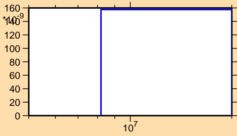
\sigma vs. E for ^{221}\text{At}(n,\text{nd})
