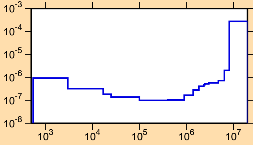
\sigma vs. E for ^{221}\text{At}(n,\alpha)
