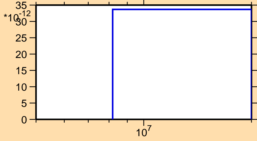
\sigma vs. E for ^{221}\text{At}(n,p\alpha)
