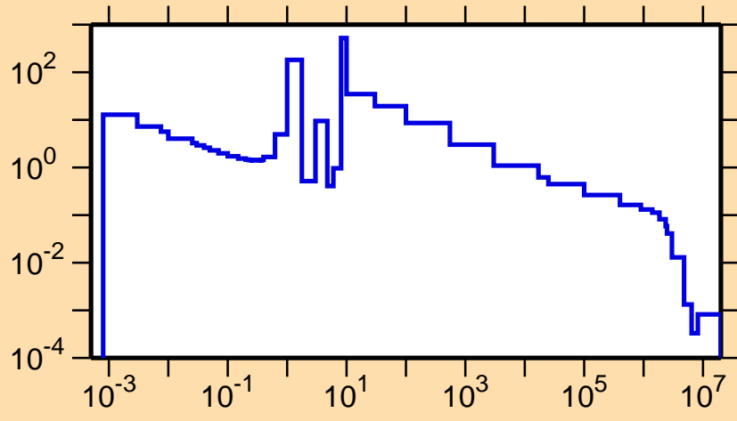
\sigma vs. E for ^{221}\text{At}(n,\gamma)
