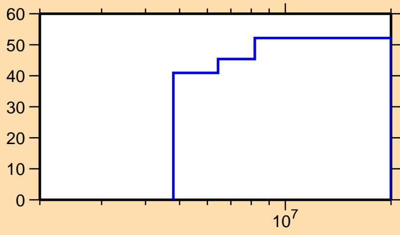
\Delta\sigma/\sigma vs. E for ^{221}\text{At}(n,\text{nonel.})
