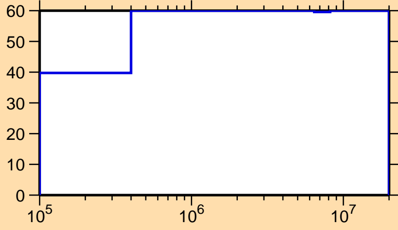
\Delta\sigma/\sigma vs. E for ^{221}\text{At}(n,n_1)
