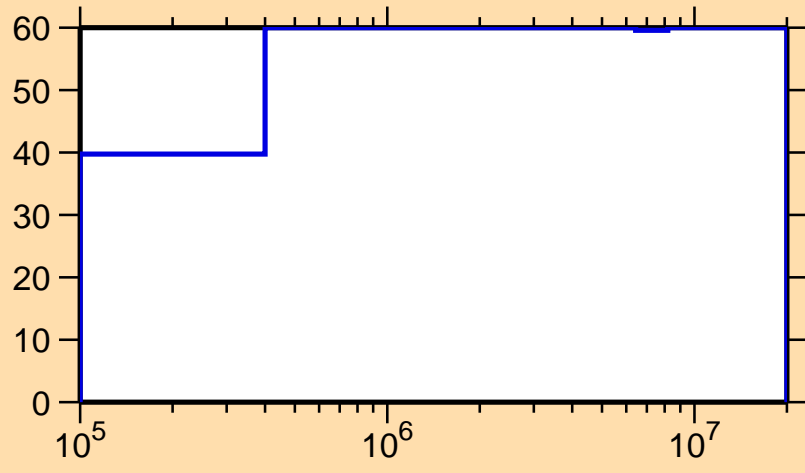
\Delta\sigma/\sigma vs. E for ^{221}\text{At}(n,n_1)
