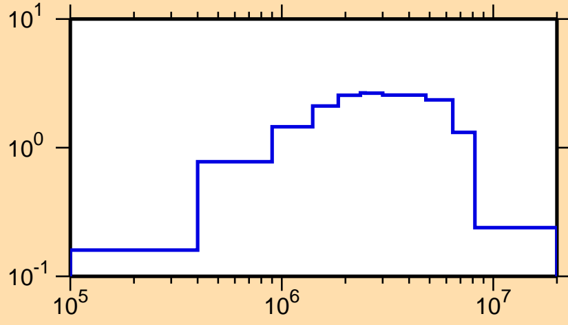
\sigma vs. E for ^{221}\text{At}(n,\text{inel.})
