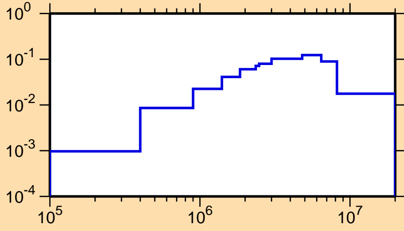
\sigma vs. E for ^{221}\text{At}(n,n\alpha)
