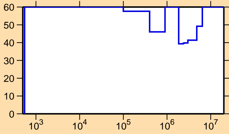
\Delta\sigma/\sigma vs. E for ^{221}\text{At}(n,\text{el.})
