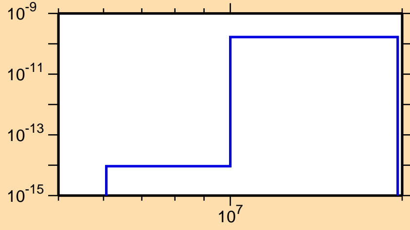
\sigma vs. E for ^{222}\text{At}(n,p\alpha)
