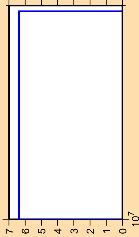
\Delta\sigma/\sigma vs. E for ^{222}\text{At}(\text{mt } 45)
