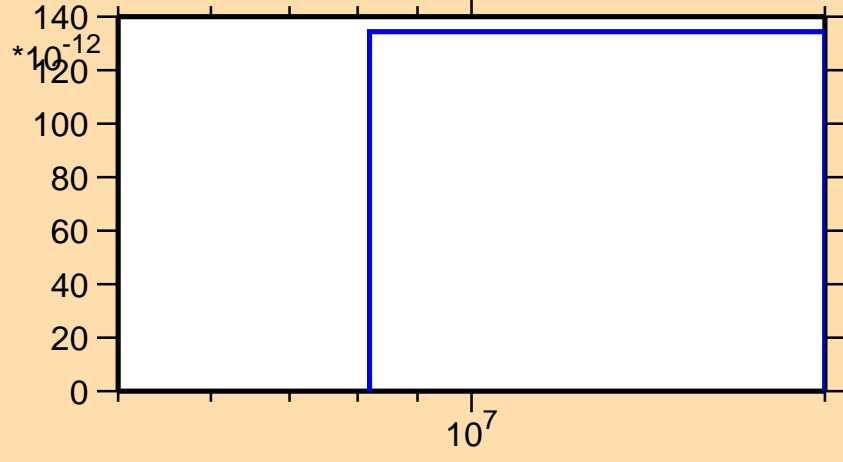
\sigma vs. E for ^{222}\text{At}(n,p\alpha)
