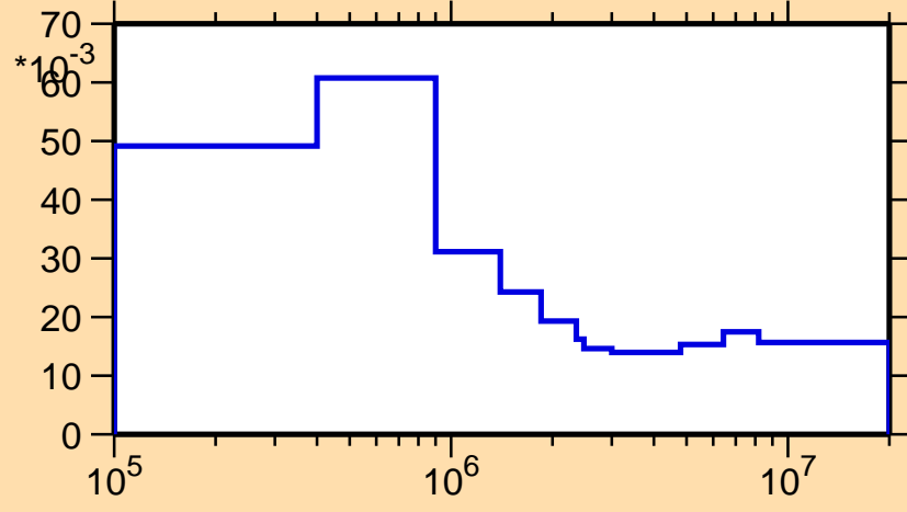
\sigma vs. E for ^{222}\text{At}(n,n_1)
