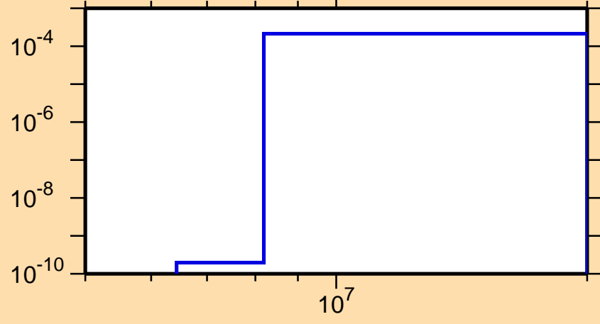
\sigma vs. E for ^{222}\text{At}(n,t)
