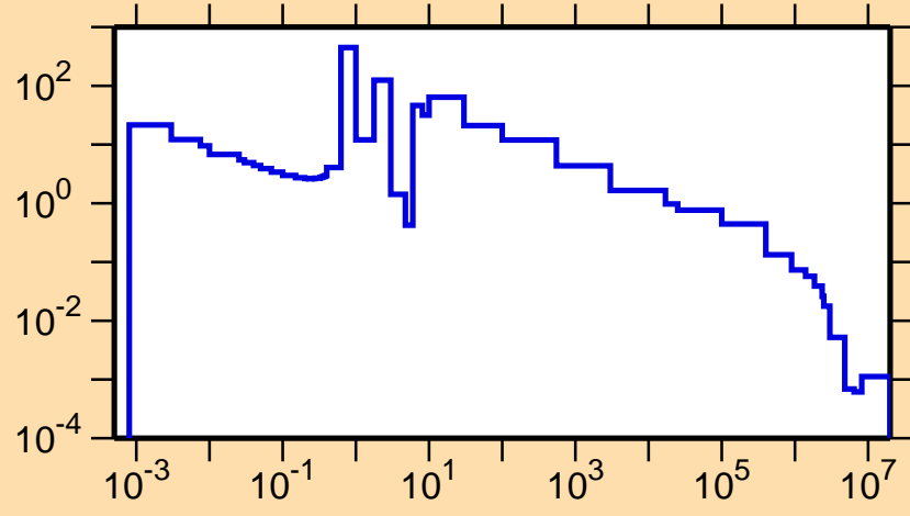
\sigma vs. E for ^{222}\text{At}(n,\gamma)
