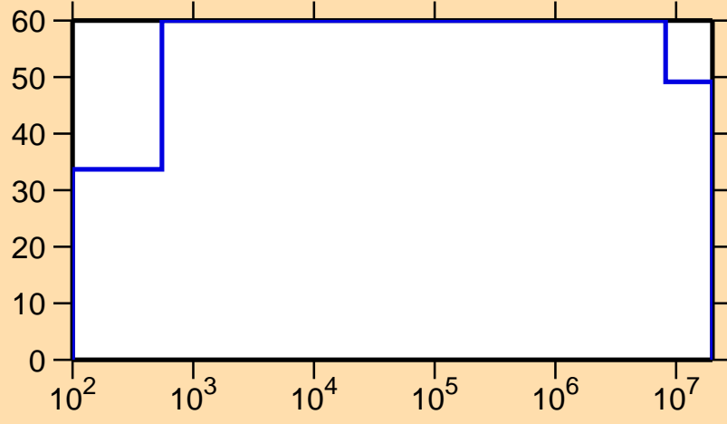
\Delta\sigma/\sigma vs. E for ^{222}\text{At}(n, \gamma)
