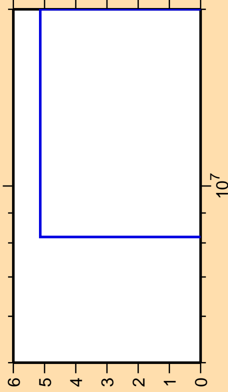
\Delta\sigma/\sigma vs. E for ^{222}\text{At}(\text{mt } 45)
