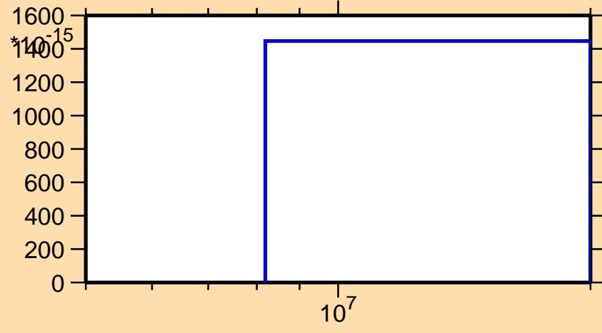
\sigma vs. E for ^{222}\text{At}(\text{mt } 45)
