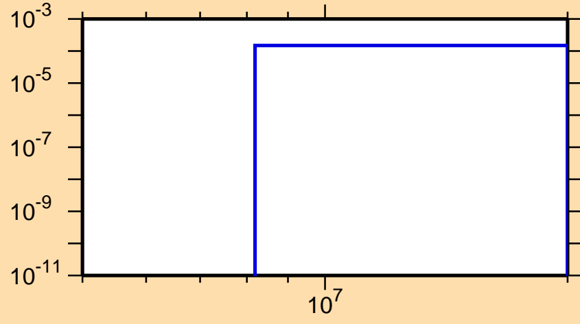
\sigma vs. E for ^{222}\text{At}(n,d)
