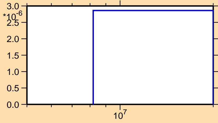
\sigma vs. E for ^{222}\text{At}(n,\text{nd})
