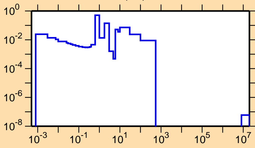
\sigma vs. E for ^{222}\text{At}(n,f)
