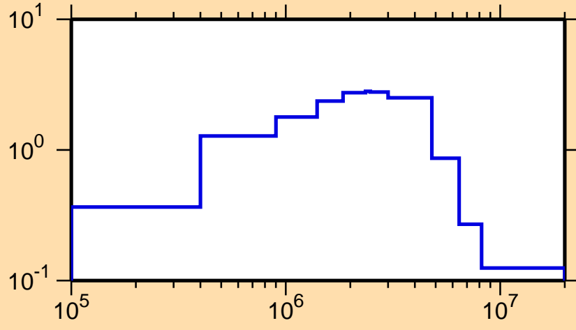
\sigma vs. E for ^{222}\text{At}(n,\text{inel.})
