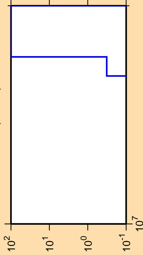
\Delta\sigma/\sigma vs. E for ^{223}\text{At} (mt 11)
