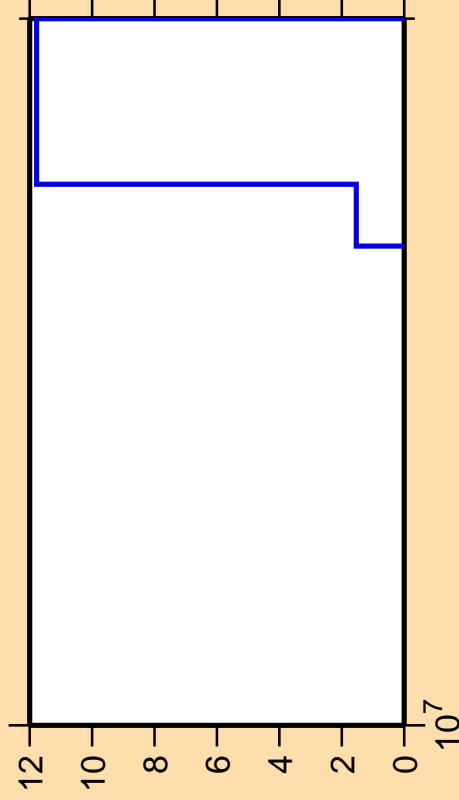
\Delta\sigma/\sigma vs. E for ^{223}\text{At}(\text{mt } 45)
