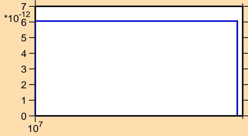
\sigma vs. E for ^{223}\text{At} (mt 11)
