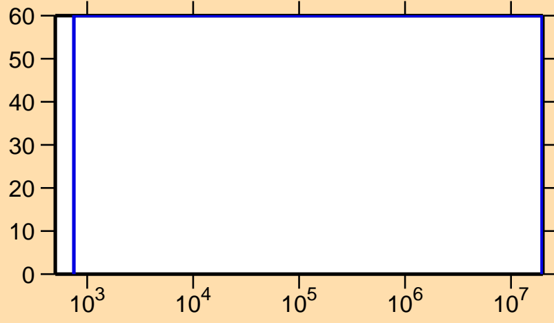
\Delta\sigma/\sigma vs. E for ^{223}\text{At}(n,\gamma)
