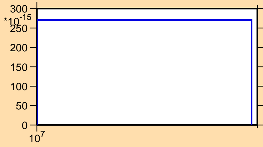
\sigma vs. E for ^{223}\text{At}(\text{mt } 42)
