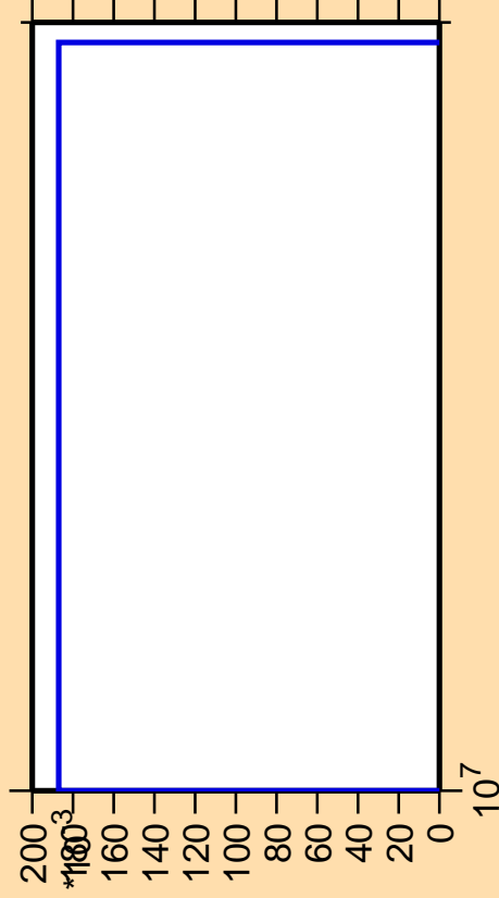
\Delta\sigma/\sigma vs. E for ^{223}\text{At}(\text{mt } 45)
