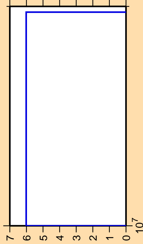
\Delta\sigma/\sigma vs. E for ^{223}\text{At} (mt 11)
