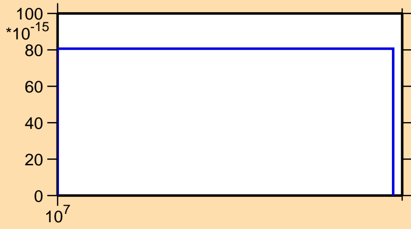
\sigma vs. E for ^{223}\text{At}(\text{mt } 45)
