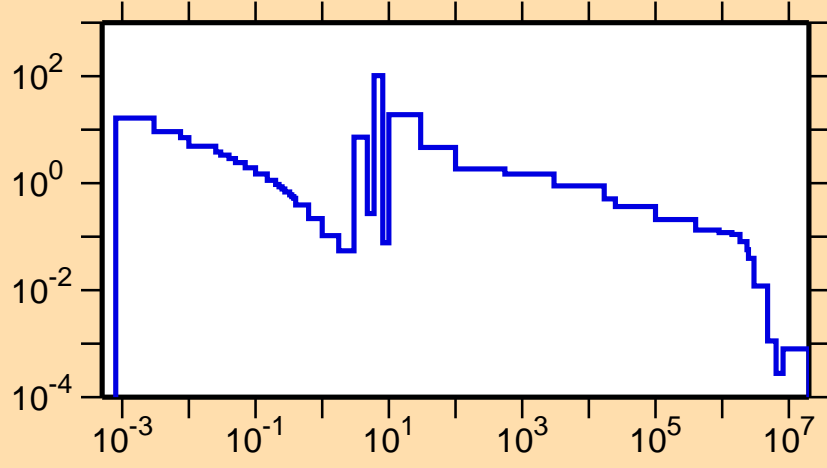
\sigma vs. E for ^{223}\text{At}(n,\gamma)
