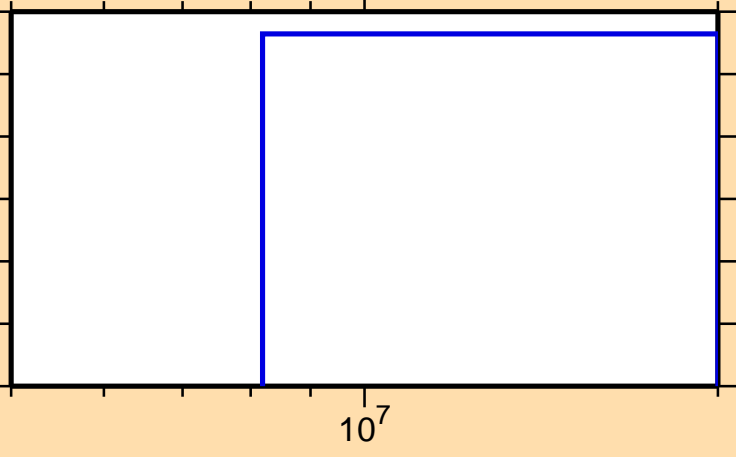
\sigma vs. E for ^{223}\text{At}(n,np)
