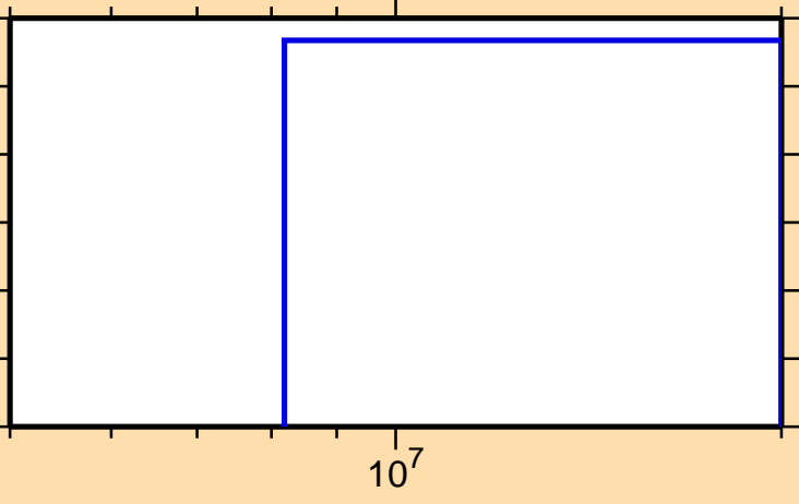
\sigma vs. E for ^{224}\text{At}(n,3n\alpha)
