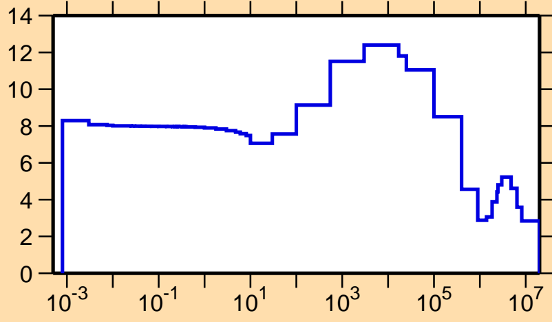
\sigma vs. E for ^{224}\text{At}(n,\text{el.})
