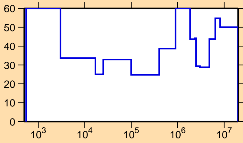
\Delta\sigma/\sigma vs. E for ^{224}\text{At}(n, \text{tot.})
