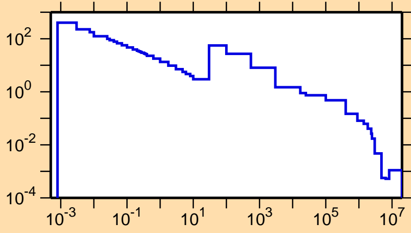
\sigma vs. E for ^{224}\text{At}(n,\gamma)
