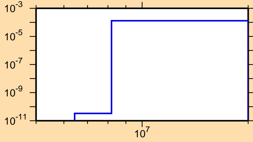
\sigma vs. E for ^{224}\text{At}(n,t)
