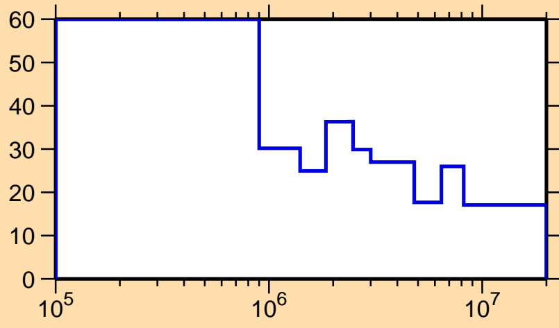
\Delta\sigma/\sigma vs. E for ^{224}\text{At}(n,\text{nonel.})
