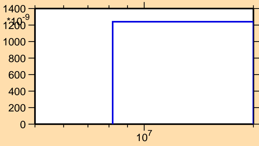
\sigma vs. E for ^{224}\text{At}(n,\text{nd})
