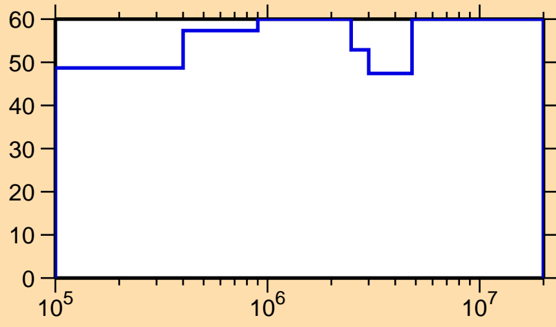
\Delta\sigma/\sigma vs. E for ^{224}\text{At}(n, \text{el.})
