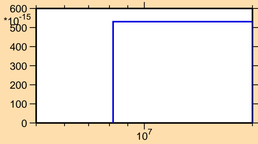
\sigma vs. E for ^{224}\text{At}(\text{mt } 42)
