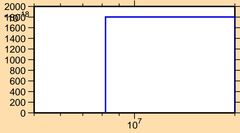
\sigma vs. E for ^{224}\text{At}(n,\text{He3})
