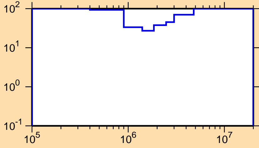
\Delta\sigma/\sigma vs. E for ^{224}\text{At}(n,n\text{cont.})
