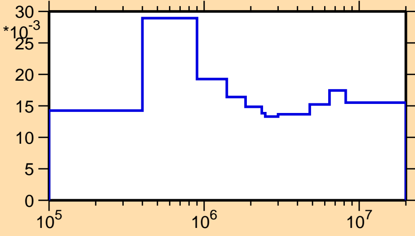
\sigma vs. E for ^{224}\text{At}(n,n_1)
