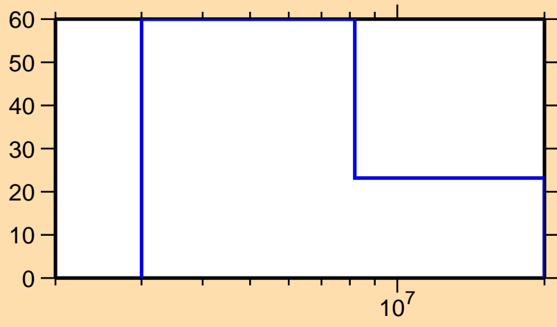
\Delta\sigma/\sigma vs. E for ^{224}\text{At}(n,2n)
