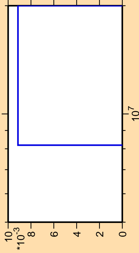
\Delta\sigma/\sigma vs. E for ^{224}\text{At}(n,\text{He3})
