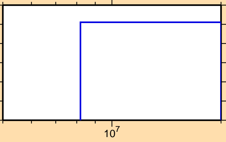
\sigma vs. E for ^{224}\text{At}(n,np)
