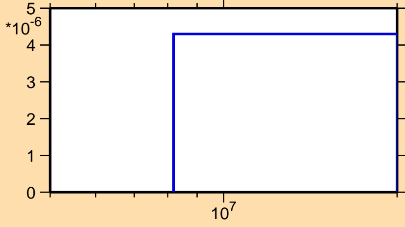
\sigma vs. E for ^{224}\text{At}(n,nt)
