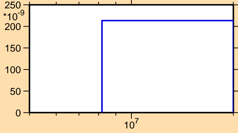
\sigma vs. E for ^{224}\text{At}(n,2np)
