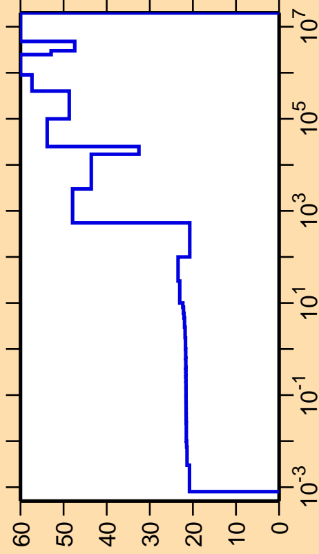
\Delta\sigma/\sigma vs. E for ^{224}\text{At}(n,\text{el.})
