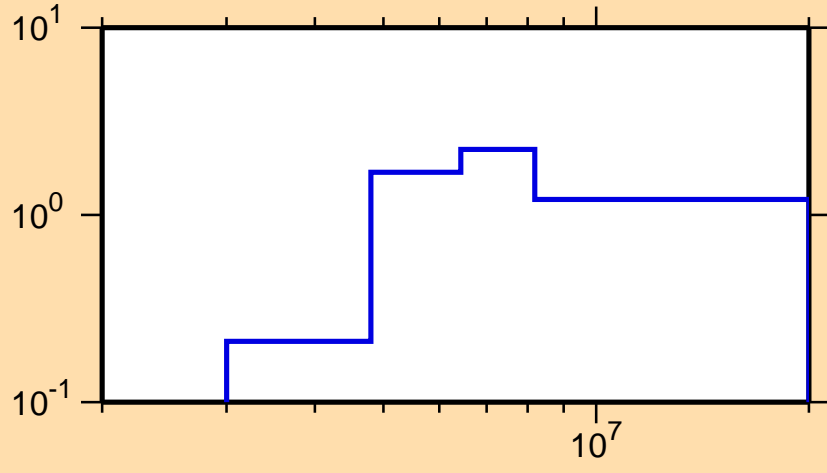
\sigma vs. E for ^{224}\text{At}(n,2n)
