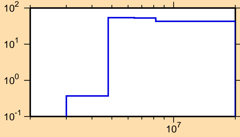
\Delta\sigma/\sigma vs. E for ^{224}\text{At}(n,p)
