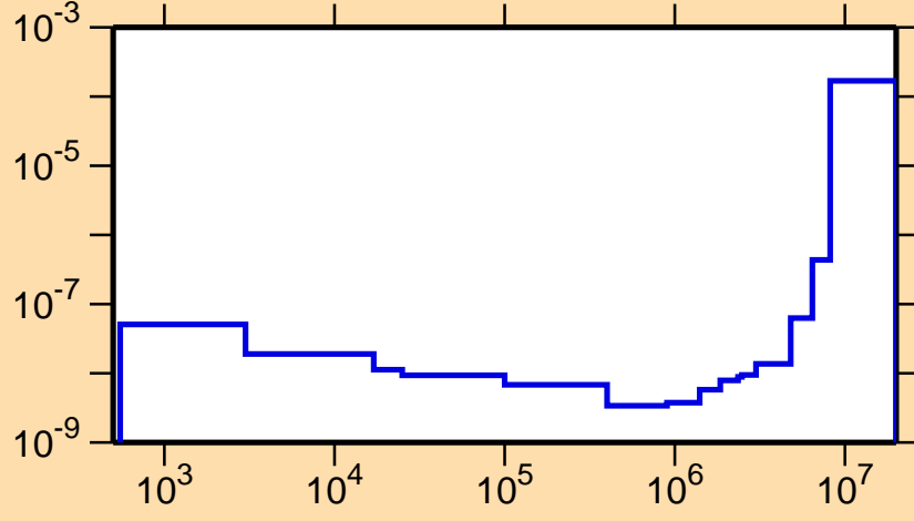
\sigma vs. E for ^{224}\text{At}(n,\alpha)
