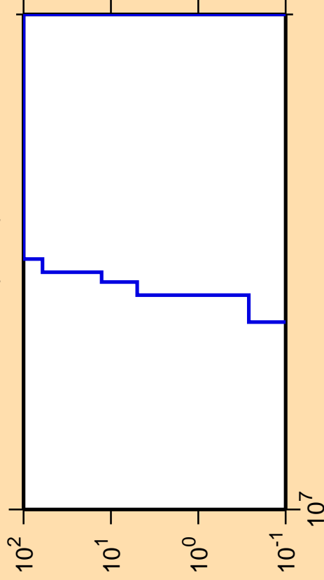
\Delta\sigma/\sigma vs. E for ^{225}\text{At}(n,\text{nd})
