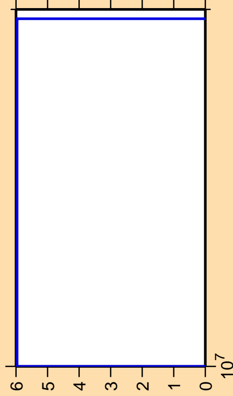
\Delta\sigma/\sigma vs. E for ^{225}\text{At} (mt 11)
