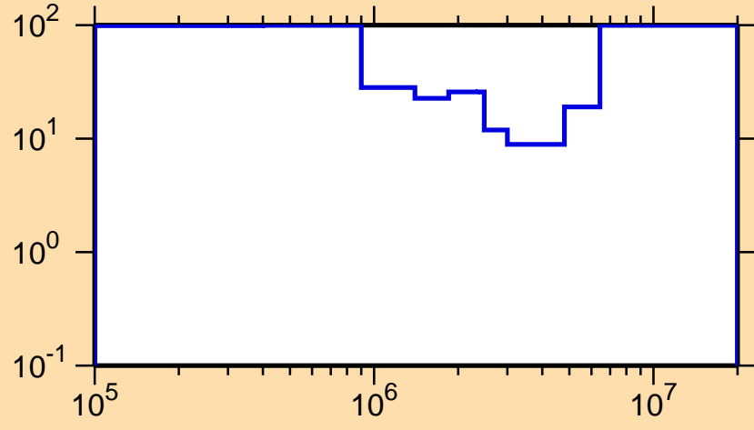
\Delta\sigma/\sigma vs. E for ^{225}\text{At}(n, inel.)
