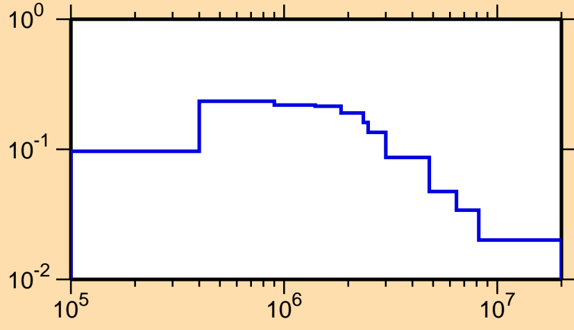
\sigma vs. E for ^{225}\text{At}(n,n_1)
