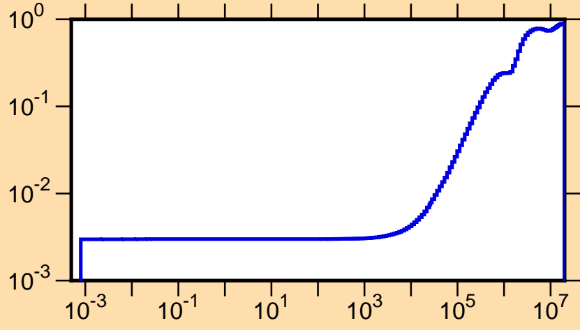
\mu vs. E for ^{226}\text{At}(\text{mt251})
