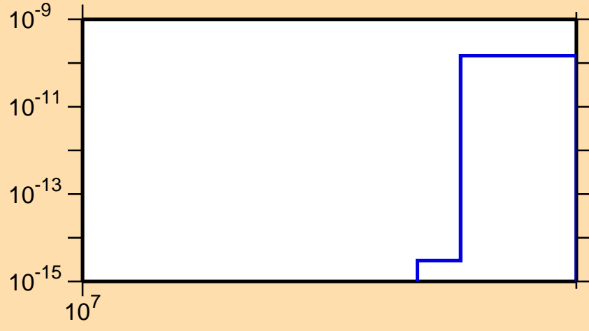
\sigma vs. E for ^{226}\text{At}(\text{mt } 11)
