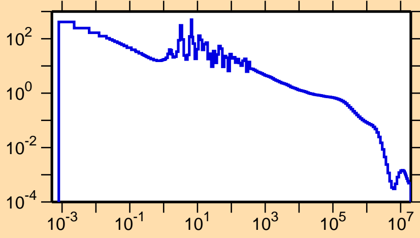
\sigma vs. E for ^{226}\text{At}(n,\gamma)
