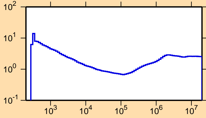
\sigma vs. E for ^{226}\text{At}(n,\text{nonel.})
