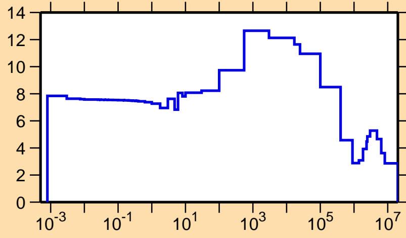
\sigma vs. E for ^{226}\text{At}(n,\text{el.})
