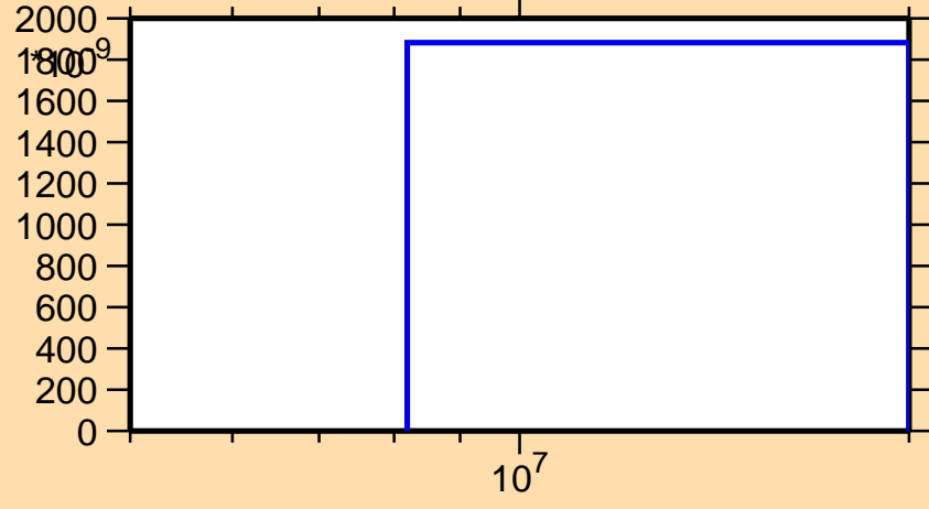
\sigma vs. E for ^{226}\text{At}(n,nt)
