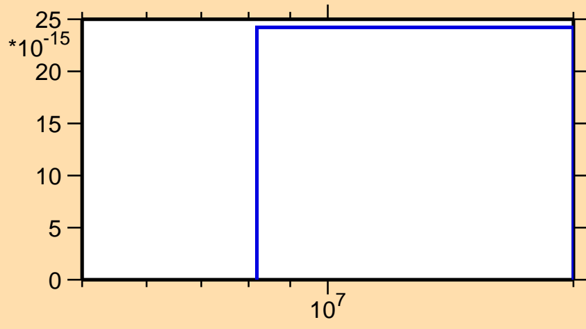
\sigma vs. E for ^{227}\text{At}(\text{mt } 42)
