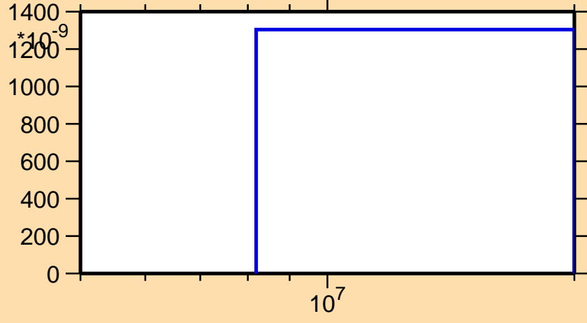
\sigma vs. E for ^{227}\text{At}(n,nt)
