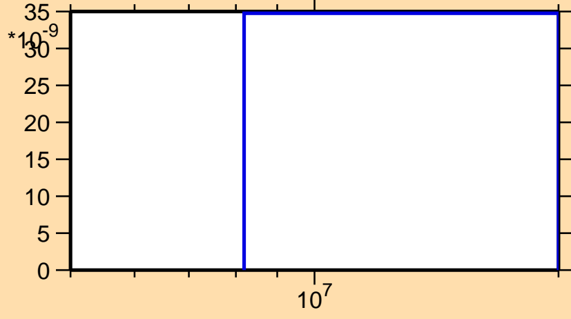
\sigma vs. E for ^{227}\text{At}(n,2n\alpha)
