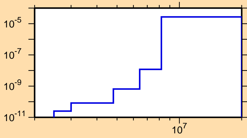
\sigma vs. E for ^{227}\text{At}(n,\alpha)
