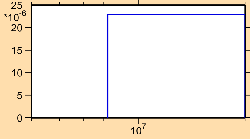
\sigma vs. E for ^{227}\text{At}(n,d)
