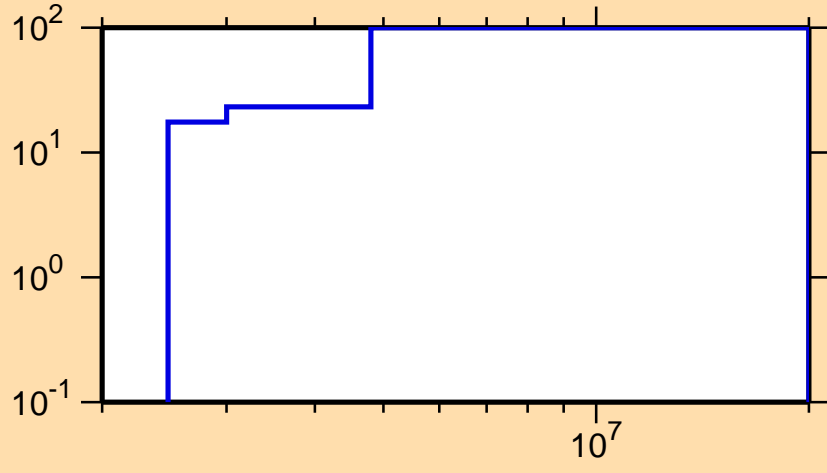
\Delta\sigma/\sigma vs. E for ^{227}\text{At}(n,ncont.)
