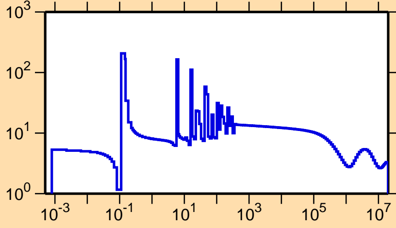
\sigma vs. E for ^{228}\text{At}(n,\text{el.})
