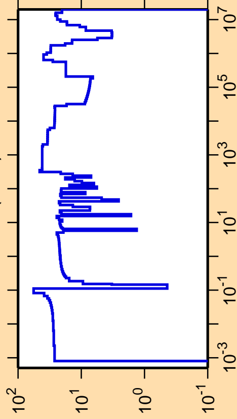
\Delta\sigma/\sigma vs. E for ^{228}\text{At}(n,\text{el.})
