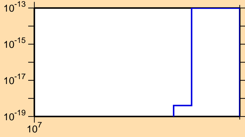
\sigma vs. E for ^{228}\text{At}(\text{mt } 42)
