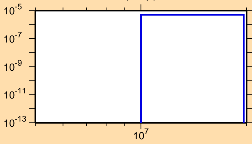
\sigma vs. E for ^{228}\text{At}(n,np)
