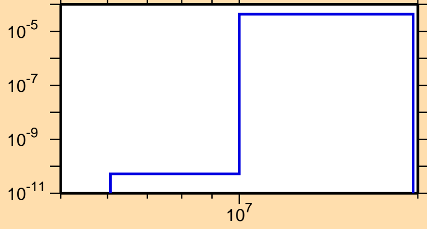
\sigma vs. E for ^{228}\text{At}(n,t)
