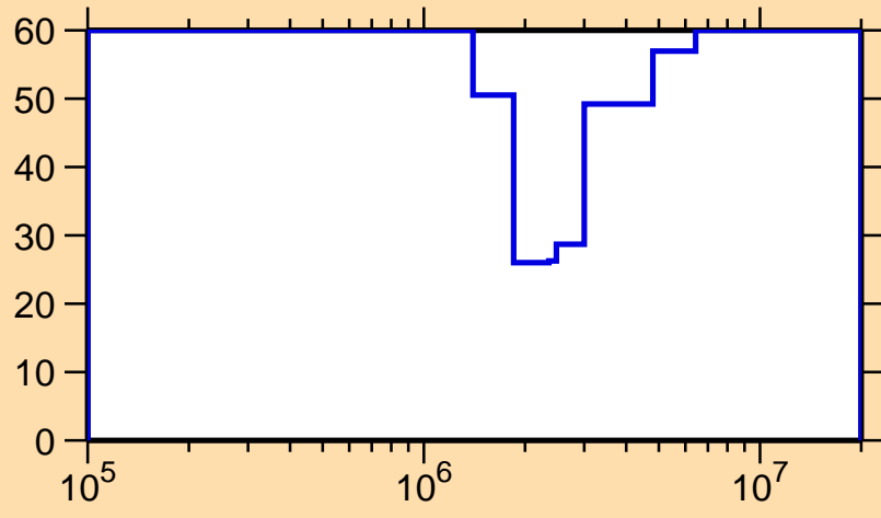
\Delta\sigma/\sigma vs. E for ^{228}\text{At}(n,n_1)
