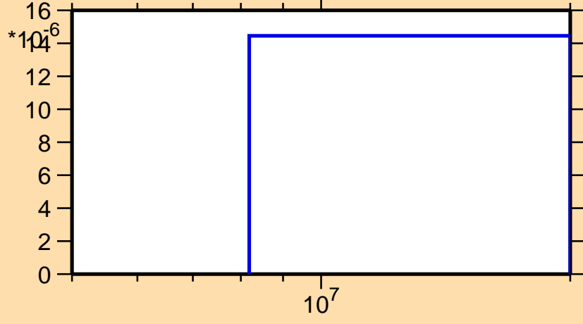
\sigma vs. E for ^{228}\text{At}(n,d)
