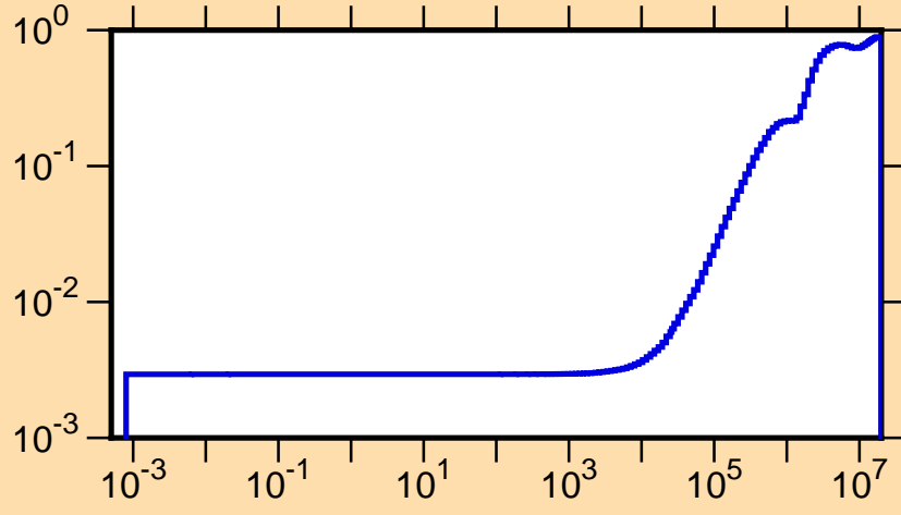
\mu vs. E for ^{229}\text{At}(\text{mt251})
