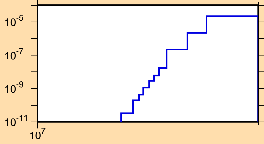
\sigma vs. E for ^{229}\text{At}(n,nt)
