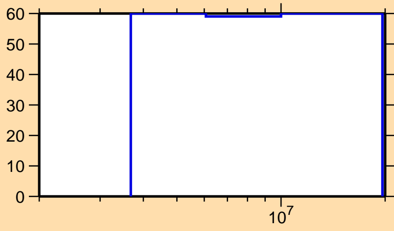
\Delta\sigma/\sigma vs. E for ^{229}\text{At}(n,2n)
