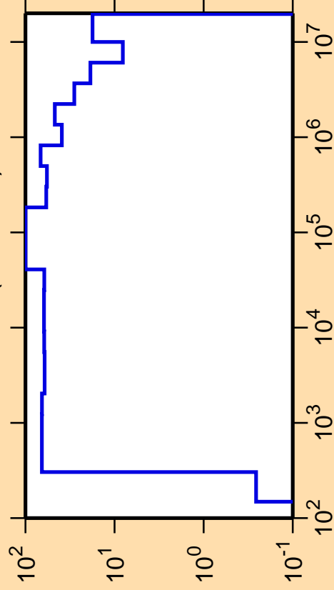
\Delta\sigma/\sigma vs. E for ^{229}\text{At}(n,\text{nonel.})
