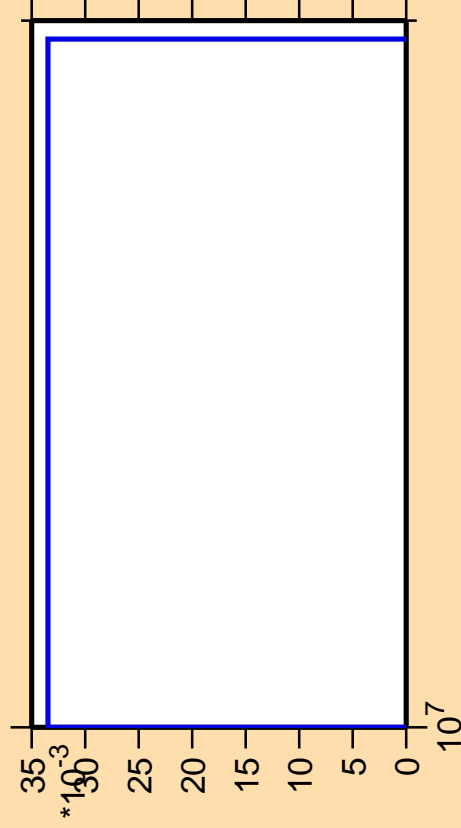
\Delta\sigma/\sigma vs. E for ^{229}\text{At}(\text{mt } 11)
