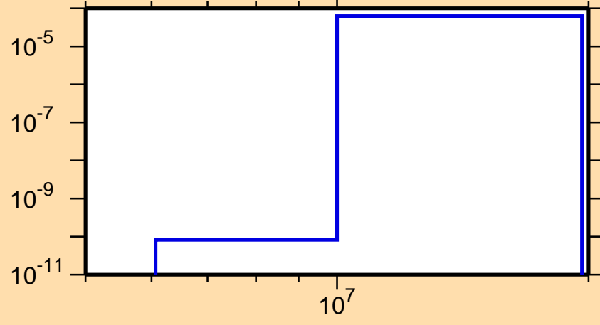
\sigma vs. E for ^{229}\text{At}(n,p)
