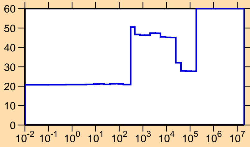
\Delta\sigma/\sigma vs. E for ^{229}\text{At}(n,el.)
