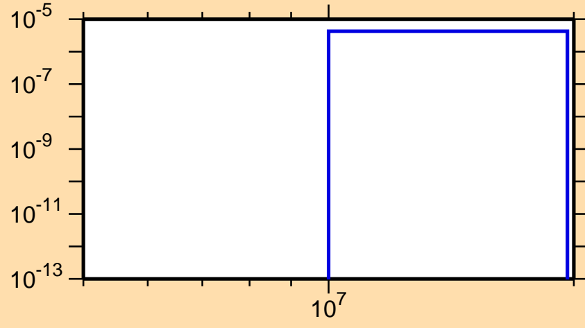
\sigma vs. E for ^{229}\text{At}(n,np)
