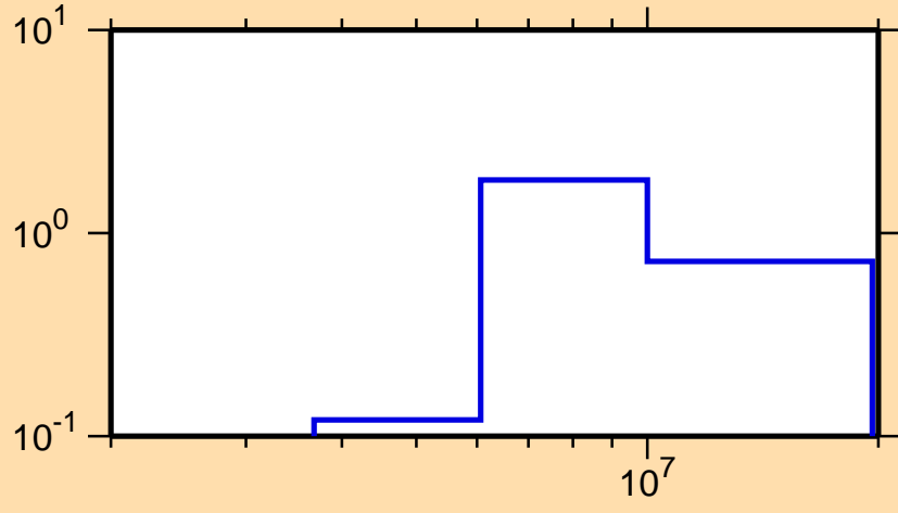
\sigma vs. E for ^{229}\text{At}(n,2n)
