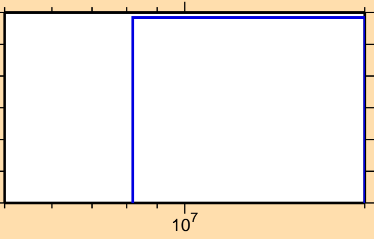
\sigma vs. E for ^{229}\text{At}(n,nt)
