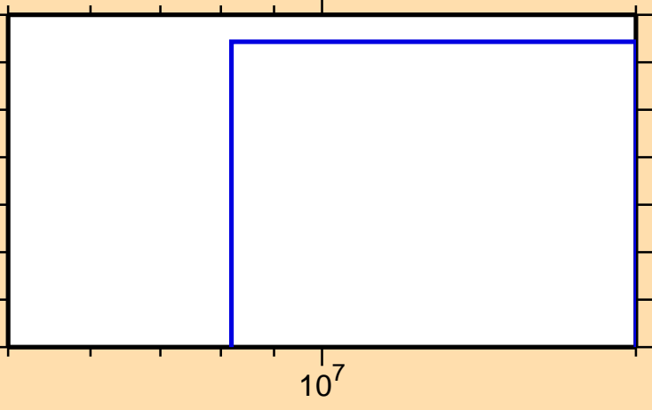
\sigma vs. E for ^{229}\text{At}(n,t)
