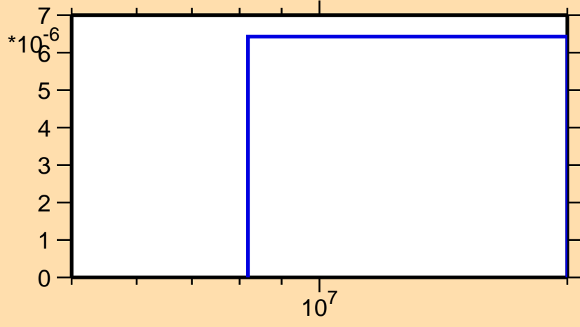
\sigma vs. E for ^{229}\text{At}(n,d)
