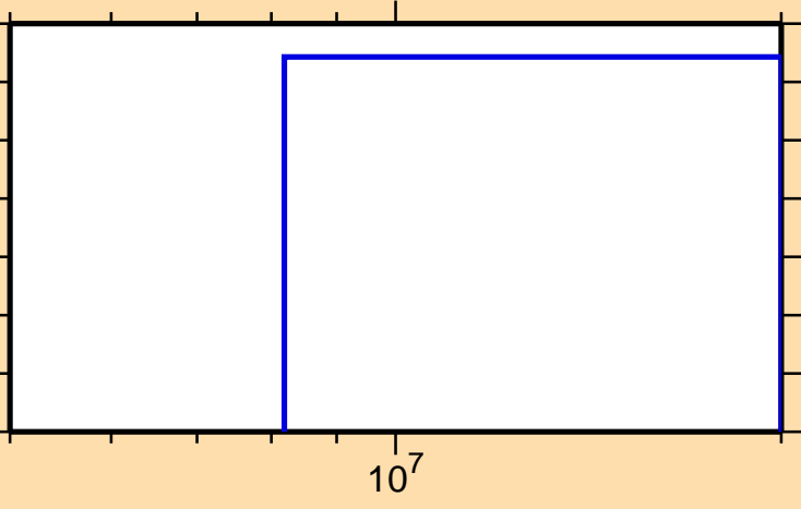
\sigma vs. E for ^{229}\text{At}(n,d)
