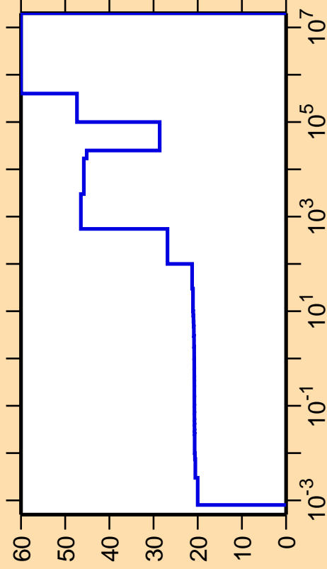
\Delta\sigma/\sigma vs. E for ^{229}\text{At}(n,\text{el.})
