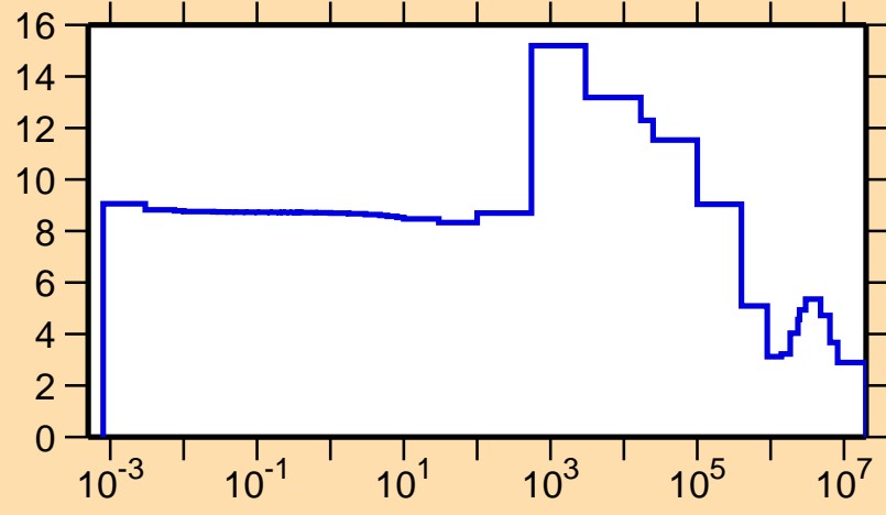
\sigma vs. E for ^{229}\text{At}(n,\text{el.})
