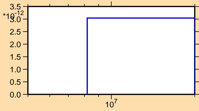
\sigma vs. E for ^{229}\text{At}(n,3n\alpha)
