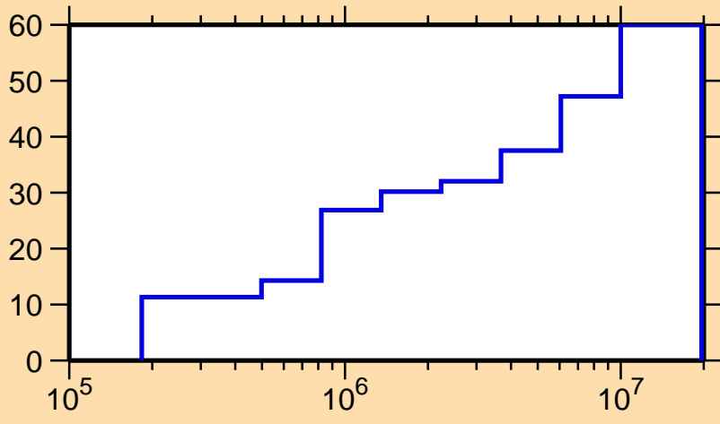
\Delta\sigma/\sigma vs. E for ^{176}\text{Au}(n,n_1)
