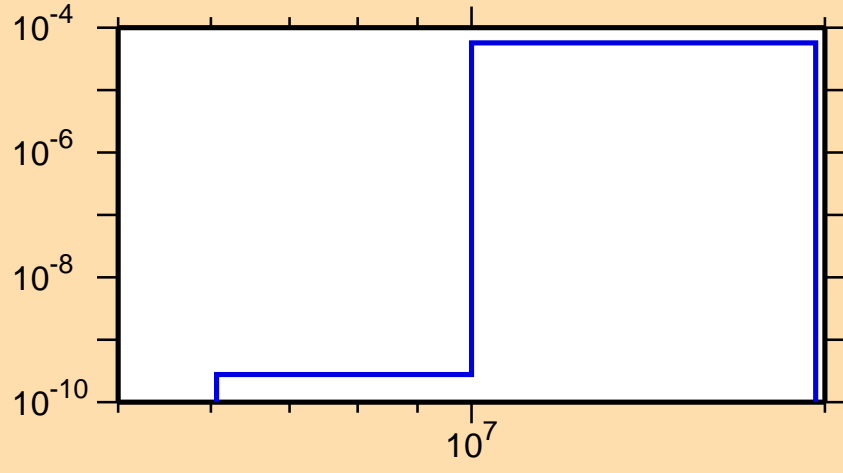
\sigma vs. E for ^{176}\text{Au}(n,\text{pd})
