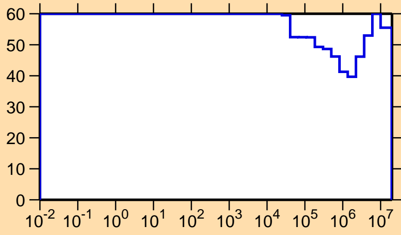
\Delta\sigma/\sigma vs. E for ^{176}\text{Au}(n,p)
