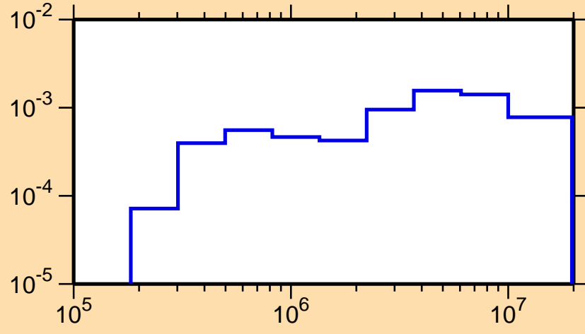
\sigma vs. E for ^{176}\text{Au}(n,n_3)
