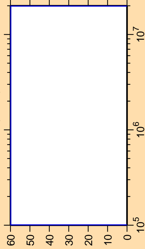
\Delta\sigma/\sigma vs. E for ^{176}\text{Au}(n,n\alpha)
