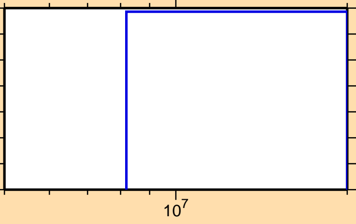
\sigma vs. E for ^{176}\text{Au}(n,2n\alpha)
