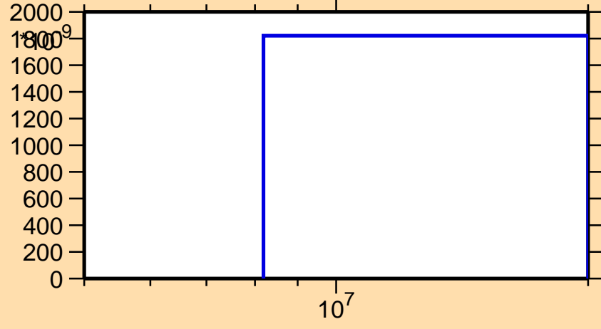
\sigma vs. E for ^{176}\text{Au}(n,pt)
