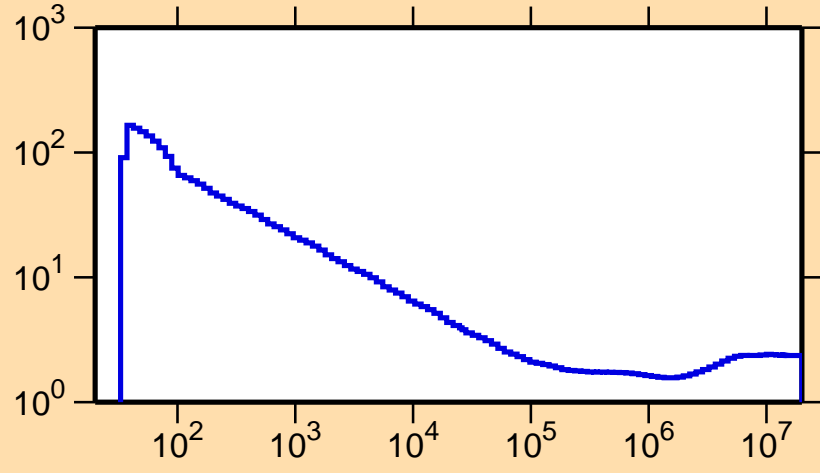
\sigma vs. E for ^{177}\text{Au}(n,\text{nonel.})
