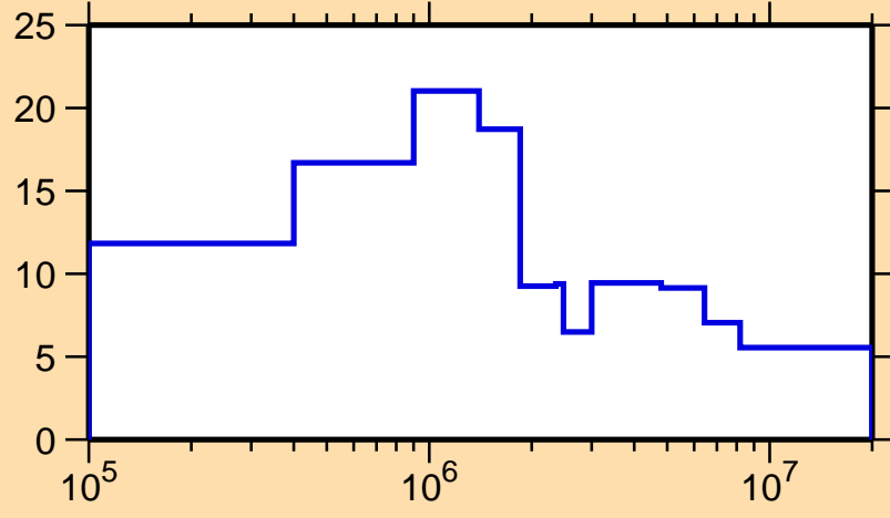
\Delta\sigma/\sigma vs. E for ^{177}\text{Au}(n,\text{tot.})
