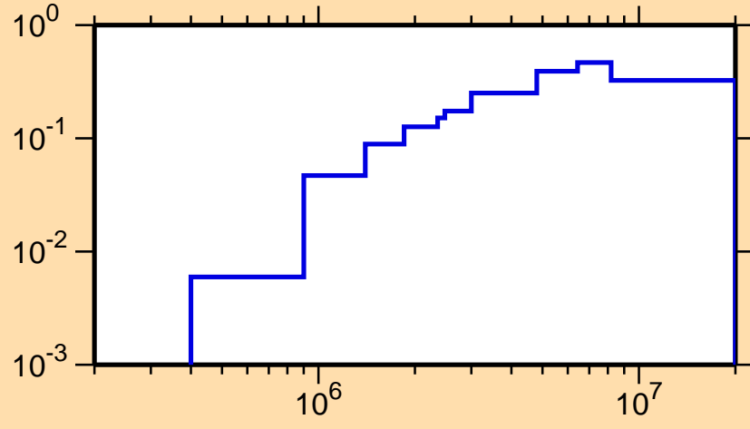
\sigma vs. E for ^{177}\text{Au}(n,n\text{cont.})
