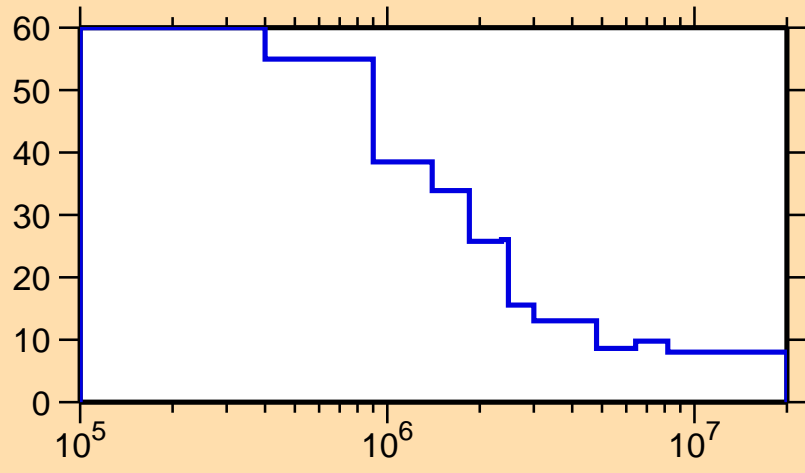
\Delta\sigma/\sigma vs. E for ^{177}\text{Au}(n,\text{nonel.})
