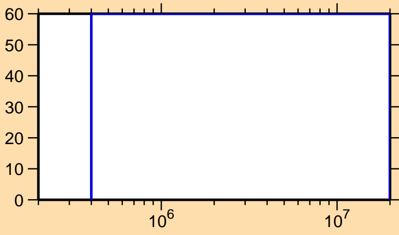
\Delta\sigma/\sigma vs. E for ^{177}\text{Au}(n,n\text{cont.})
