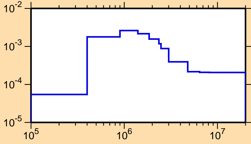
\sigma vs. E for ^{177}\text{Au}(n,n_2)
