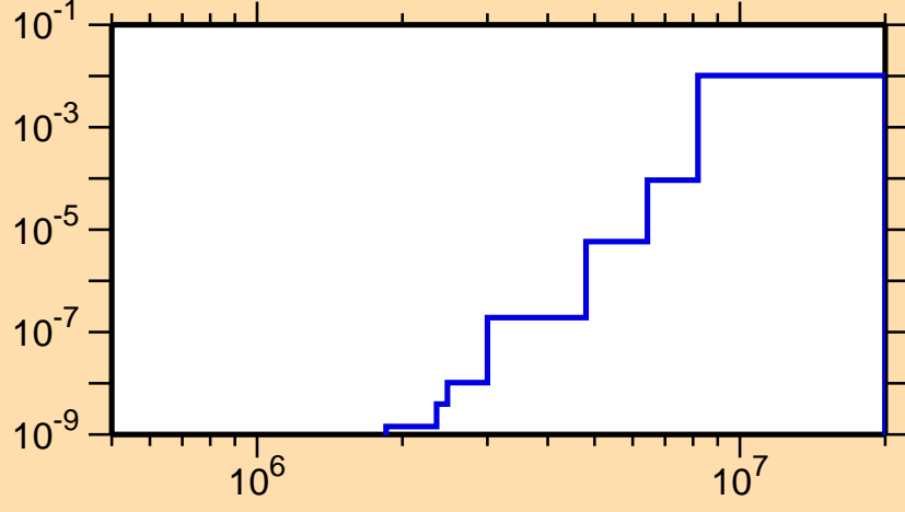
\sigma vs. E for ^{177}\text{Au}(n,d)
