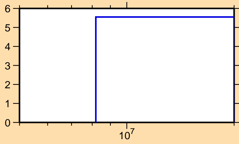
\Delta\sigma/\sigma vs. E for ^{177}\text{Au}(n,\text{tot.})
