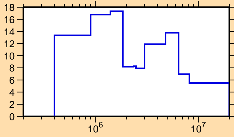
\Delta\sigma/\sigma vs. E for ^{177}\text{Au}(n, el.)
