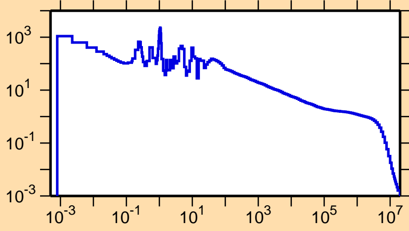
\sigma vs. E for ^{179}\text{Au}(n,\gamma)
