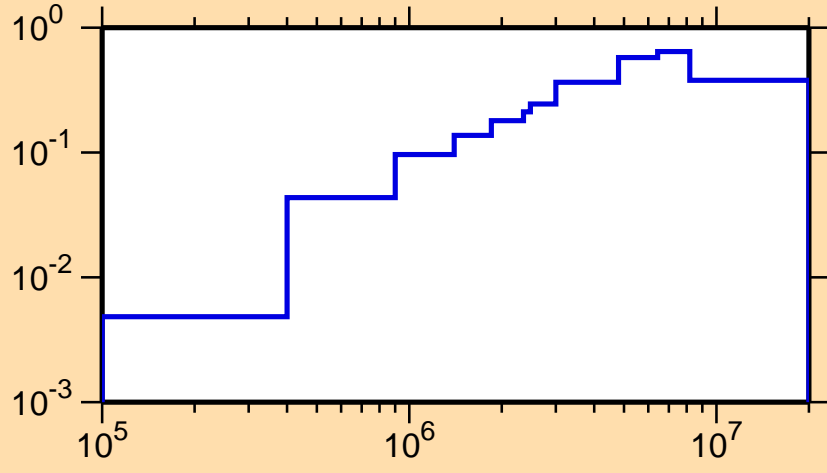
\sigma vs. E for ^{179}\text{Au}(n,n\text{cont.})
