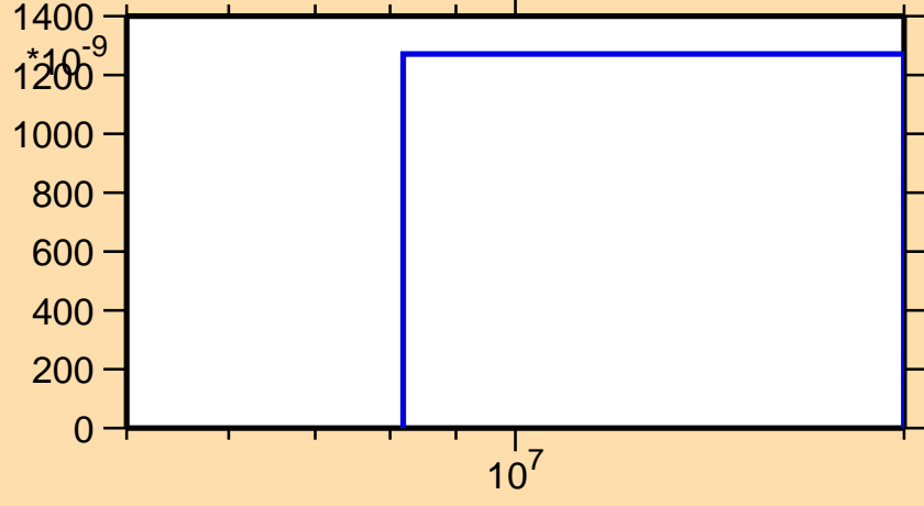
\sigma vs. E for ^{179}\text{Au}(n,pd)
