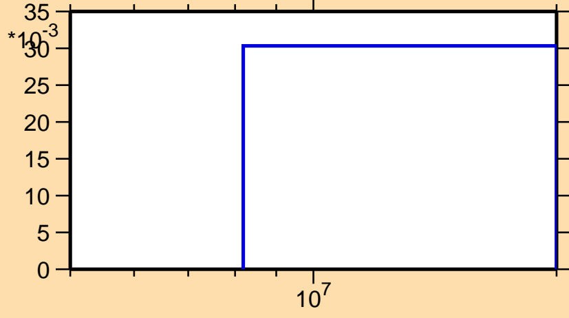
\sigma vs. E for ^{179}\text{Au}(n,2n\alpha)
