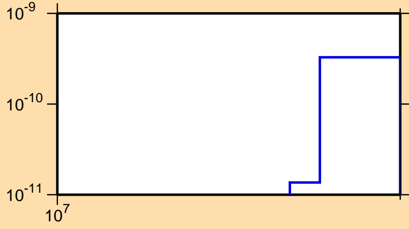
\sigma vs. E for ^{181}\text{Au} (mt 34)
