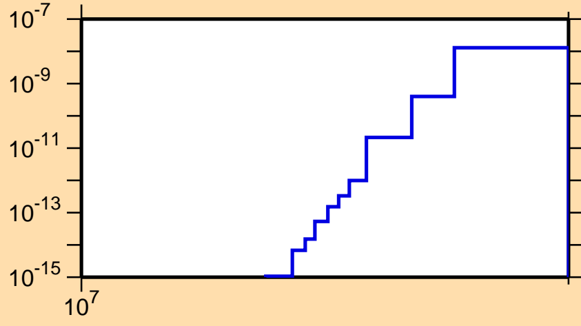
\sigma vs. E for ^{181}\text{Au}(n,pt)
