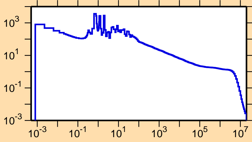
\sigma vs. E for ^{181}\text{Au}(n,\gamma)
