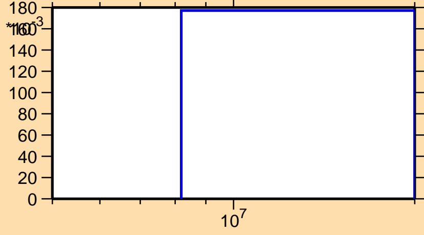
\sigma vs. E for ^{181}\text{Au}(n,2n)
