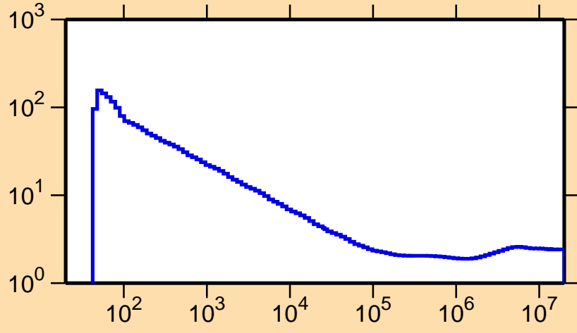
\sigma vs. E for ^{183}\text{Au}(n,\text{nonel.})
