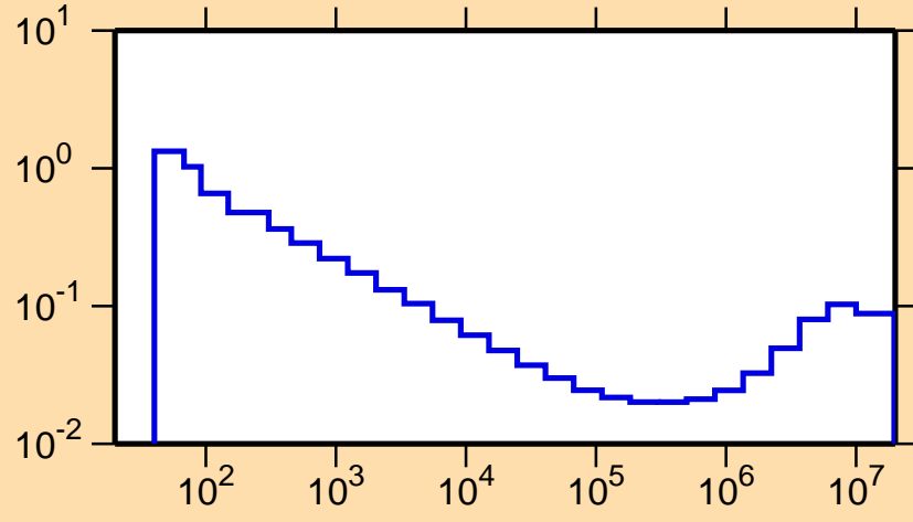
\sigma vs. E for ^{183}\text{Au}(n,p)
