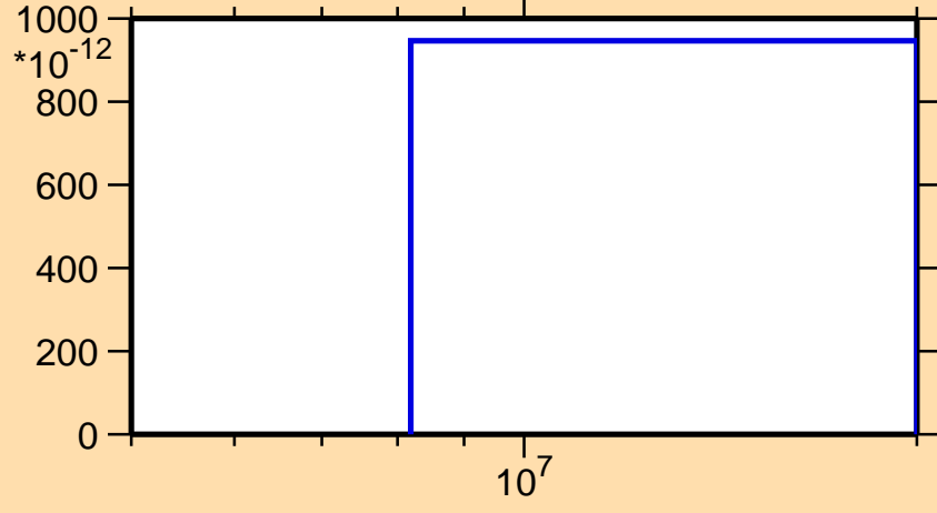
\sigma vs. E for ^{183}\text{Au}(n,nt)
