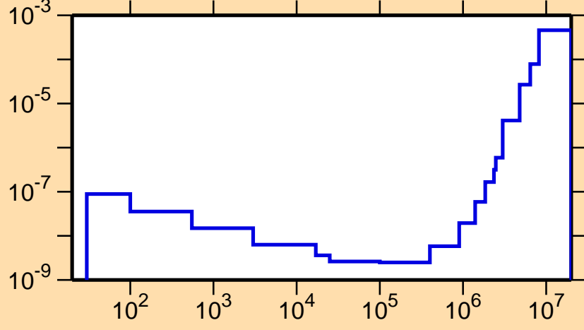
\sigma vs. E for ^{183}\text{Au}(n,p\alpha)
