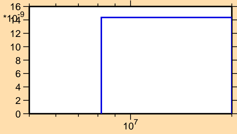
\sigma vs. E for ^{183}\text{Au}(n,\text{pd})
