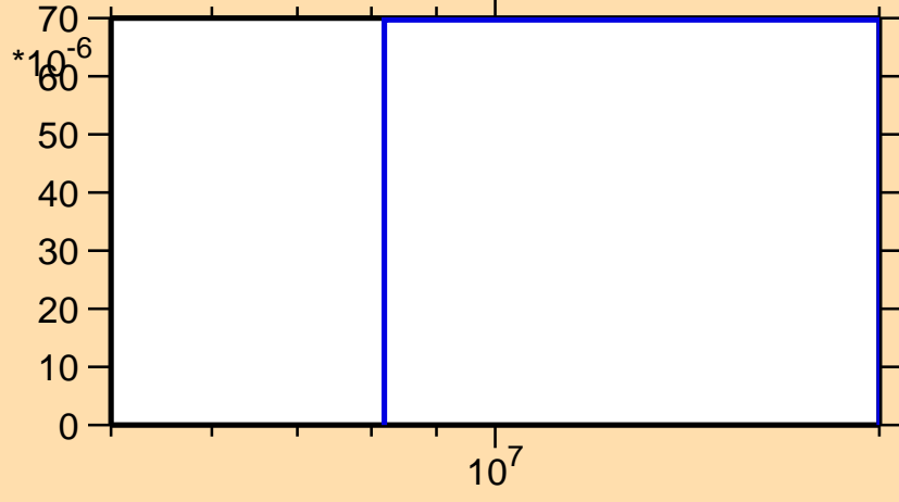
\sigma vs. E for ^{183}\text{Au}(n,2np)
