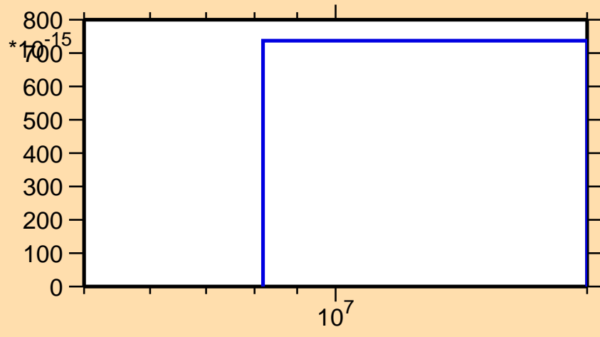
\sigma vs. E for ^{183}\text{Au}(\text{mt } 34)
