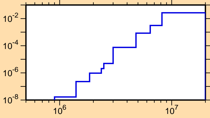
\sigma vs. E for ^{183}\text{Au}(n,n\alpha)
