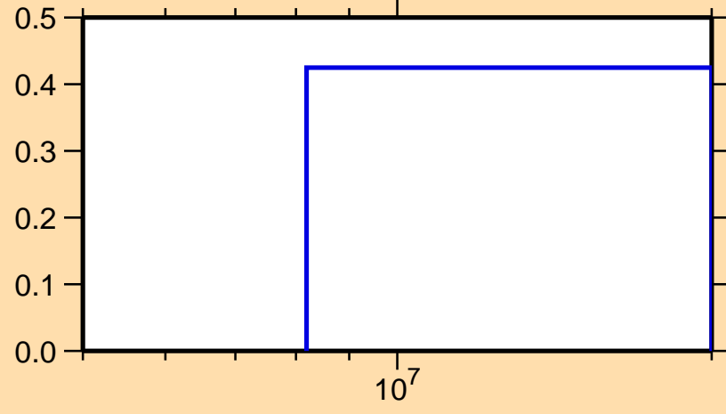
\sigma vs. E for ^{183}\text{Au}(n,2n)
