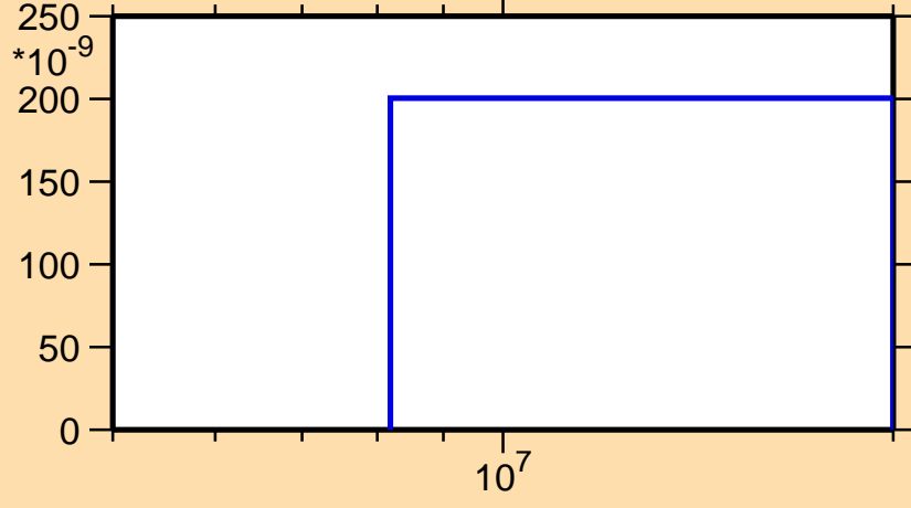
\sigma vs. E for ^{183}\text{Au}(n,3n)
