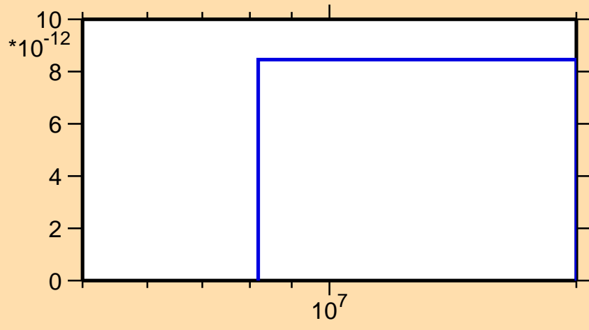
\sigma vs. E for ^{183}\text{Au}(n,\text{pt})
