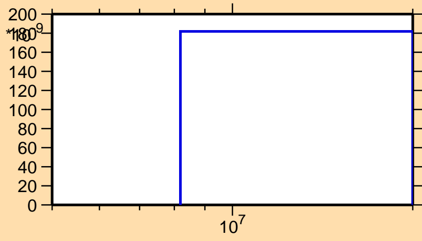
\sigma vs. E for ^{183}\text{Au}(n,\text{nd})
