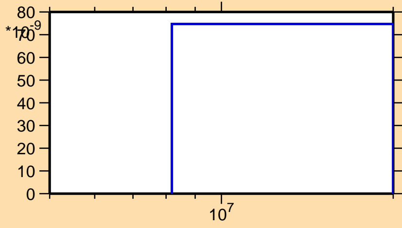
\sigma vs. E for ^{183}\text{Au}(n,3n\alpha)
