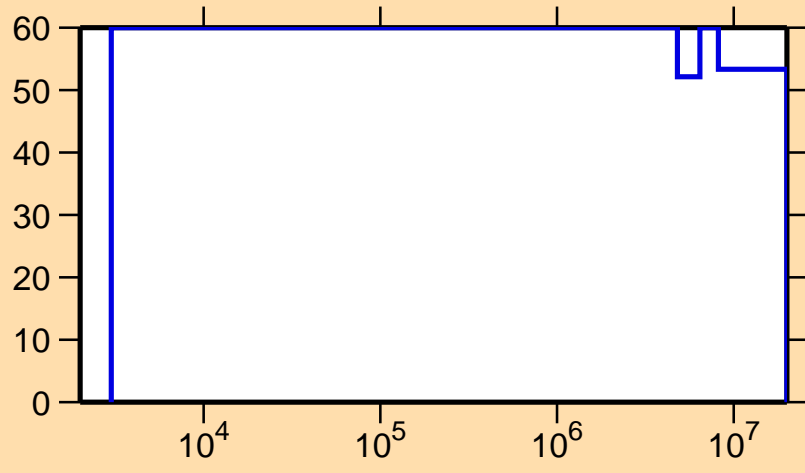
\Delta\sigma/\sigma vs. E for ^{183}\text{Au}(n,n_1)
