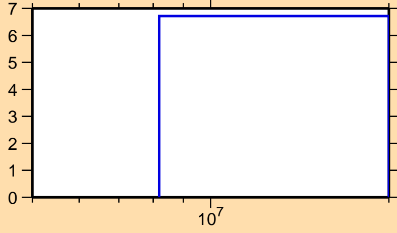
\Delta\sigma/\sigma vs. E for ^{183}\text{Au}(n,\text{el.})
