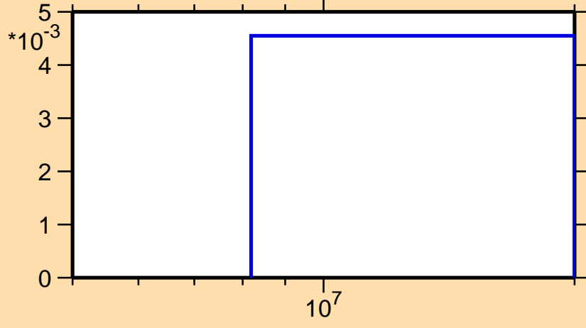
\sigma vs. E for ^{183}\text{Au}(n,2n\alpha)
