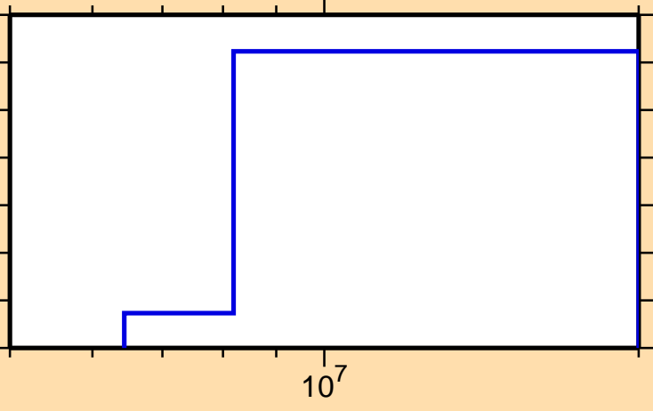
\sigma vs. E for ^{184}\text{Au}(\text{mt117})
