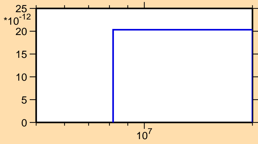
\sigma vs. E for ^{184}\text{Au}(\text{mt } 34)
