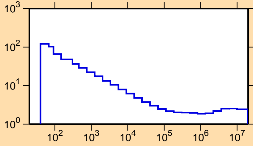
\sigma vs. E for ^{184}\text{Au}(n,\text{nonel.})
