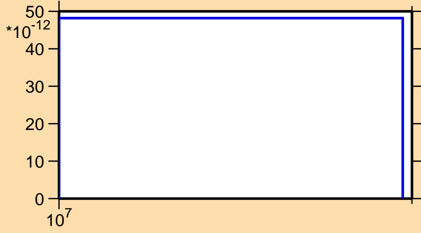
\sigma vs. E for ^{184}\text{Au} (mt 34)
