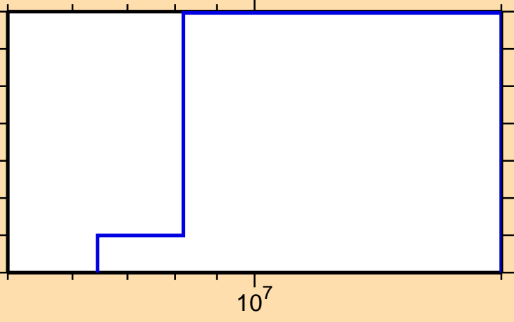
\sigma vs. E for ^{184}\text{Au}(n,2n)
