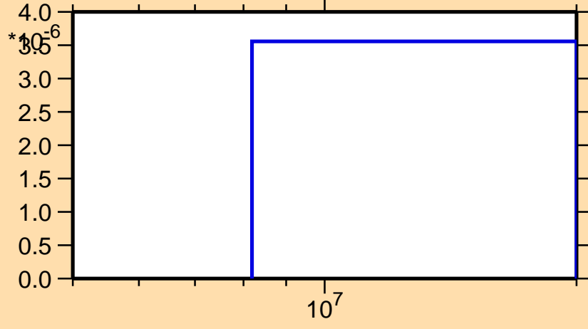
\sigma vs. E for ^{184}\text{Au}(n,nd)
