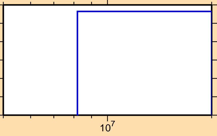
\sigma vs. E for ^{184}\text{Au}(n,\text{pd})
