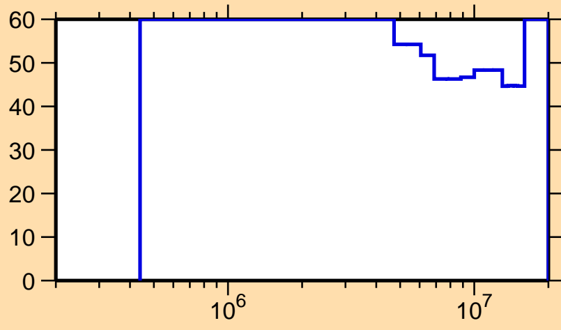
\Delta\sigma/\sigma vs. E for ^{185}\text{Au}(n,n\text{cont.})
