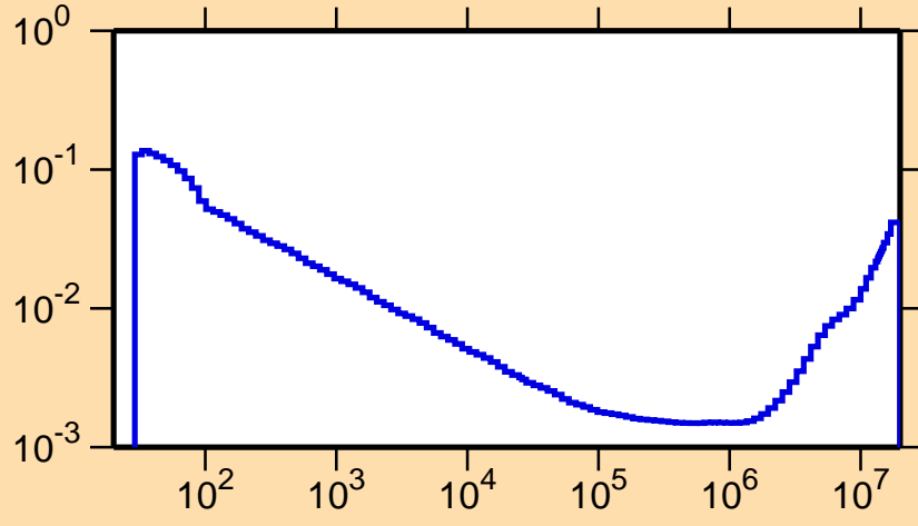
\sigma vs. E for ^{185}\text{Au}(n,\alpha)
