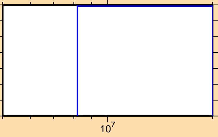
\sigma vs. E for ^{185}\text{Au}(n,2np)
