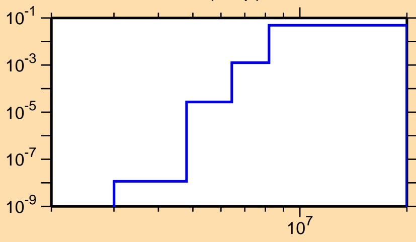
\sigma vs. E for ^{185}\text{Au}(n,np)
