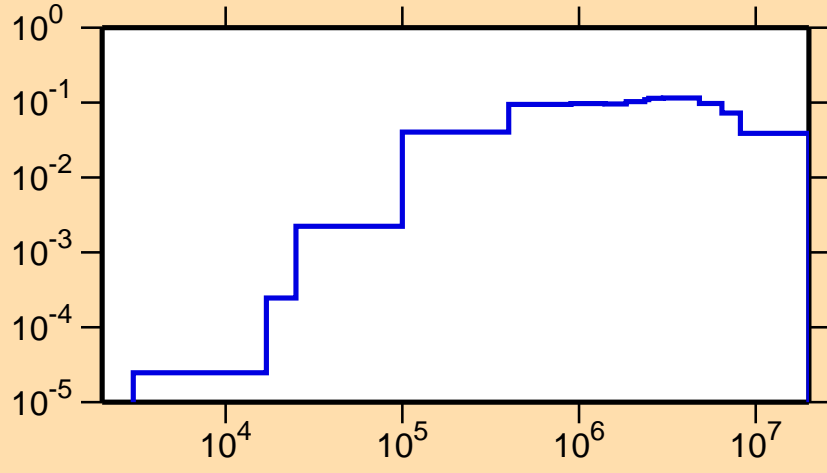
\sigma vs. E for ^{185}\text{Au}(n,n_1)
