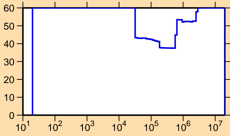
\Delta\sigma/\sigma vs. E for ^{185}\text{Au}(n,\gamma)
