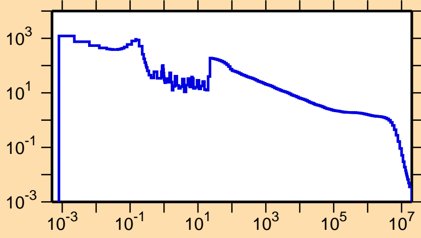
\sigma vs. E for ^{185}\text{Au}(n,\gamma)
