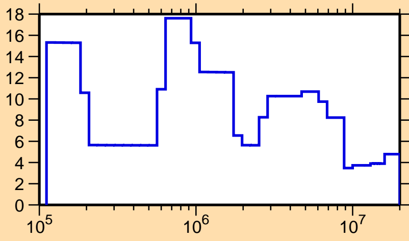
\Delta\sigma/\sigma vs. E for ^{185}\text{Au}(n,\text{tot.})
