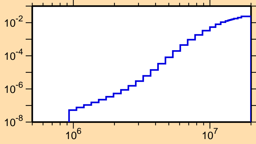
\sigma vs. E for ^{185}\text{Au}(n,n\alpha)
