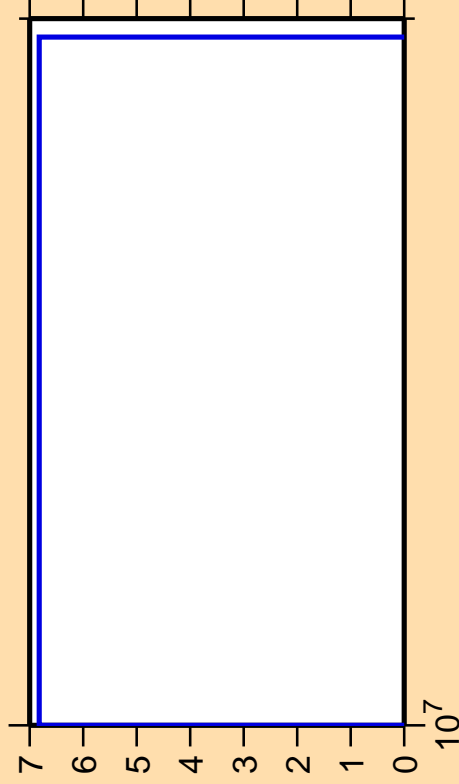
\Delta\sigma/\sigma vs. E for ^{185}\text{Au}(n,pt)
