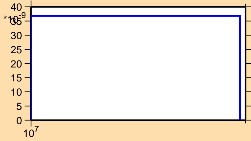
\sigma vs. E for ^{185}\text{Au}(n,3n\alpha)
