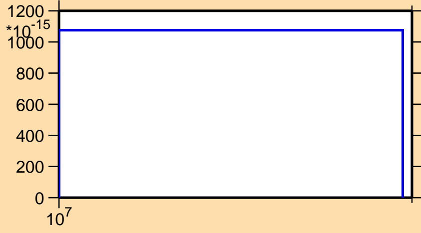
\sigma vs. E for ^{185}\text{Au}(n,pt)
