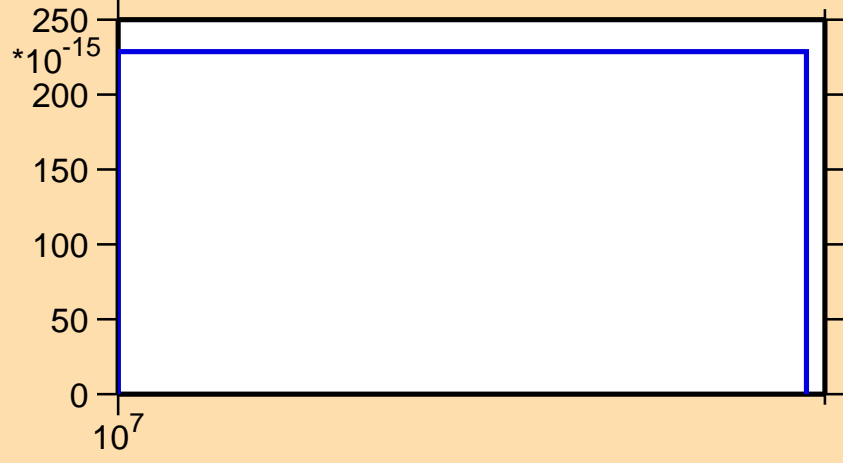
\sigma vs. E for ^{185}\text{Au} (mt 34)
