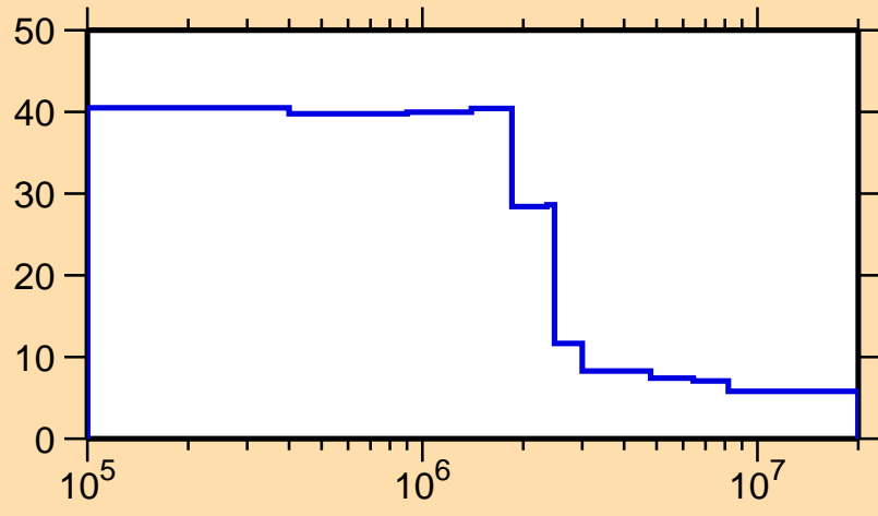
\Delta\sigma/\sigma vs. E for ^{185}\text{Au}(n,\text{nonel.})
