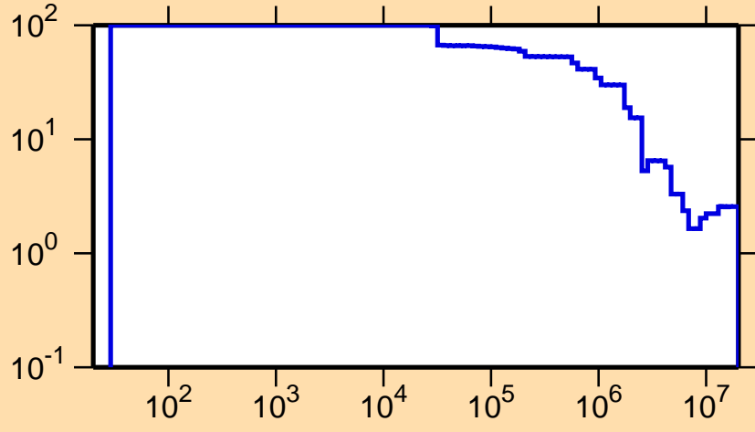
\Delta\sigma/\sigma vs. E for ^{186}\text{Au}(n,\text{nonel.})
