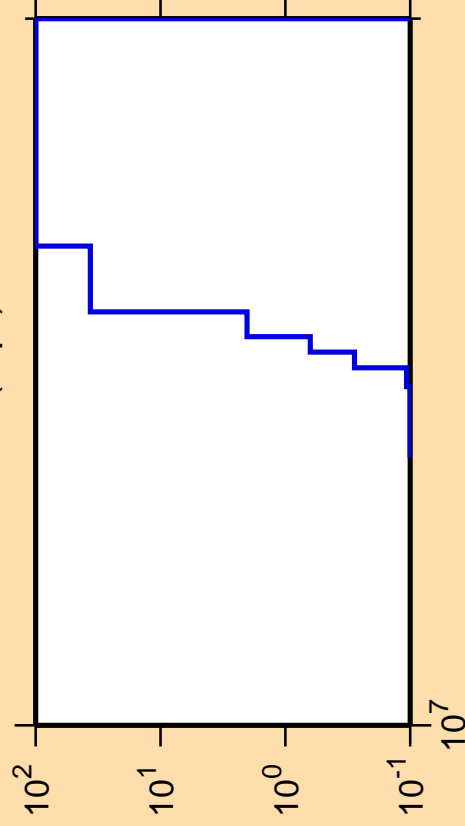
\Delta\sigma/\sigma vs. E for ^{186}\text{Au}(n,pt)
