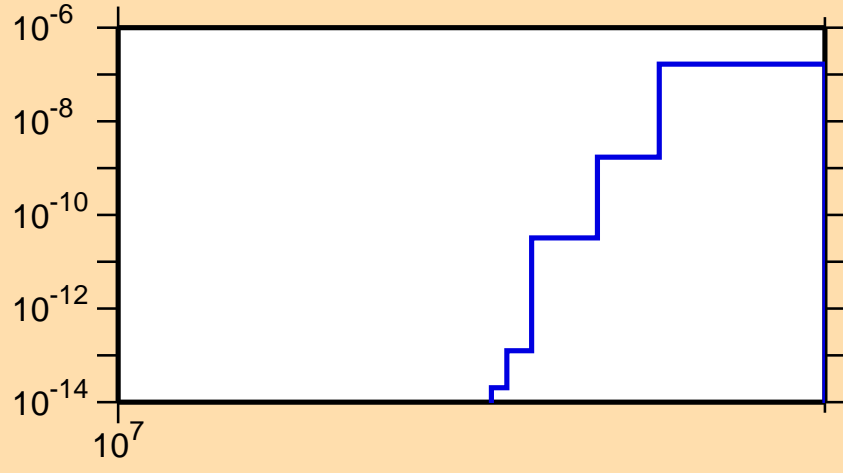
\sigma vs. E for ^{186}\text{Au}(n,nt)
