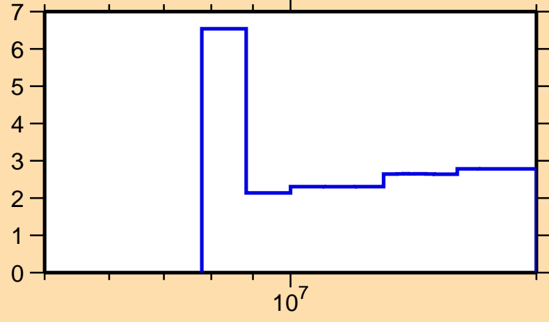
\Delta\sigma/\sigma vs. E for ^{186}\text{Au}(n,\text{tot.})
