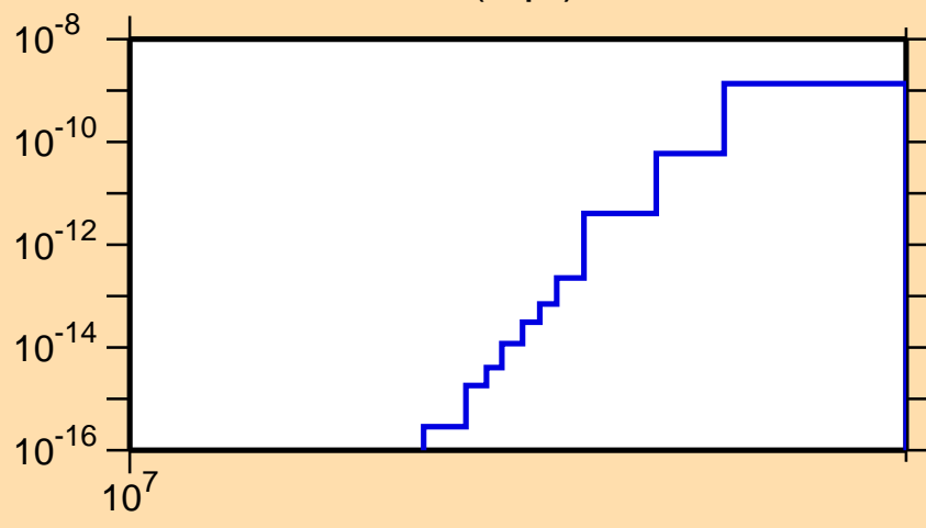
\sigma vs. E for ^{186}\text{Au}(n,pt)
