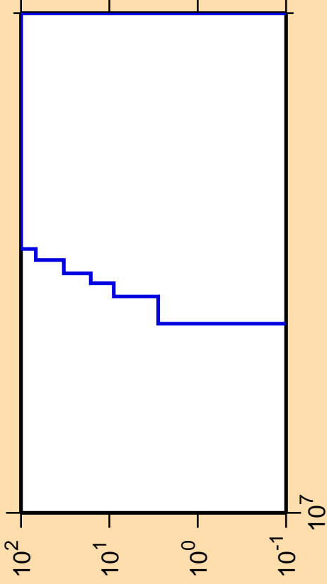
\Delta\sigma/\sigma vs. E for ^{186}\text{Au}(n,\text{pd})
