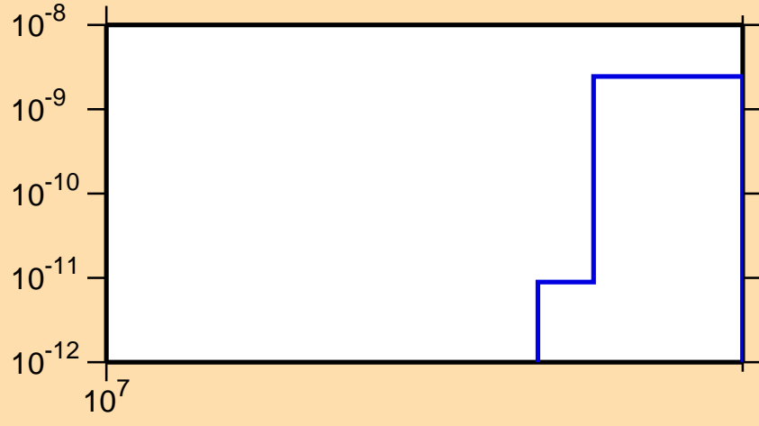
\sigma vs. E for ^{186}\text{Au}(n,3n\alpha)
