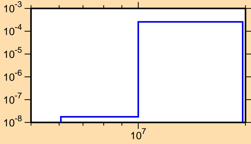
\sigma vs. E for ^{186}\text{Au}(n,2n\alpha)
