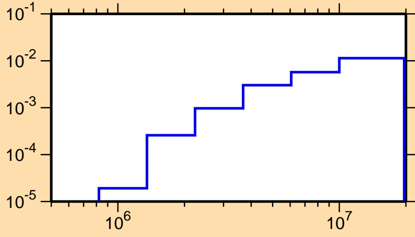
\sigma vs. E for ^{186}\text{Au}(n,n\alpha)
