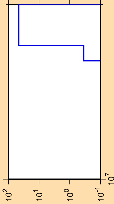
\Delta\sigma/\sigma vs. E for ^{187}\text{Au} (mt 34)
