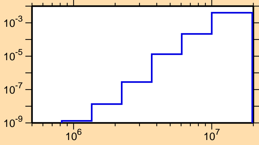
\sigma vs. E for ^{187}\text{Au}(n,n\alpha)
