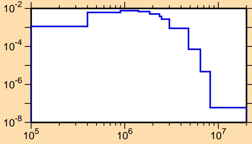
\sigma vs. E for ^{187}\text{Au}(n,n_2)
