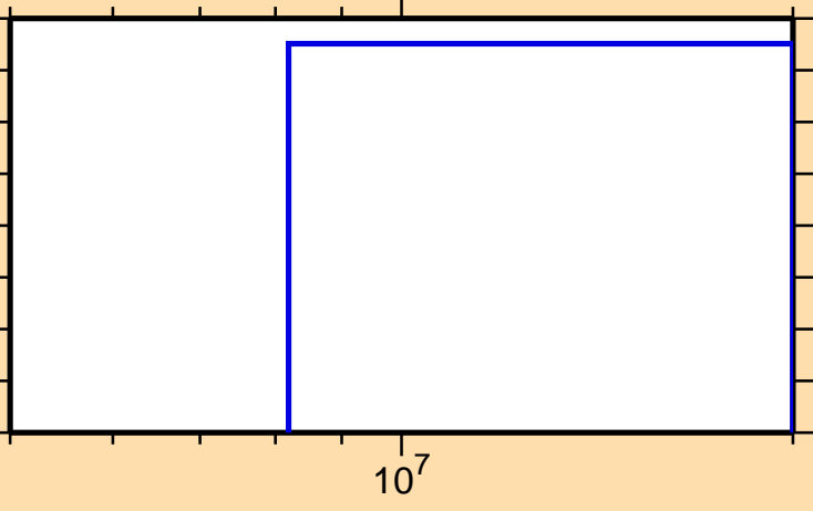
\sigma vs. E for ^{187}\text{Au}(n,2n\alpha)
