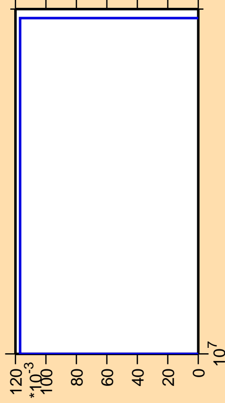
\Delta\sigma/\sigma vs. E for ^{187}\text{Au} (mt 34)
