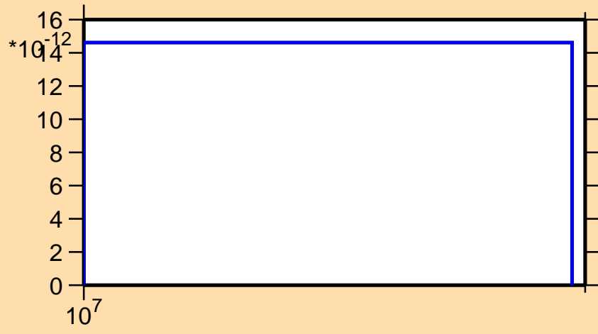
\sigma vs. E for ^{187}\text{Au}(n,3n\alpha)
