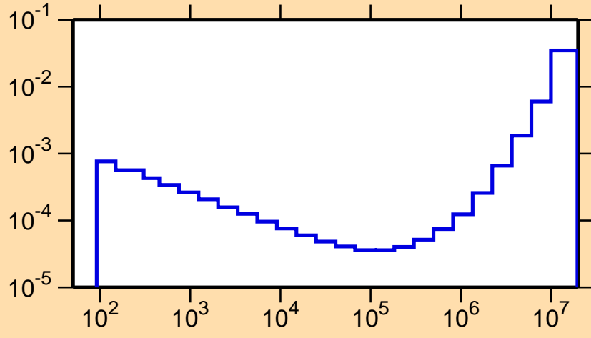
\sigma vs. E for ^{187}\text{Au}(n,p)
