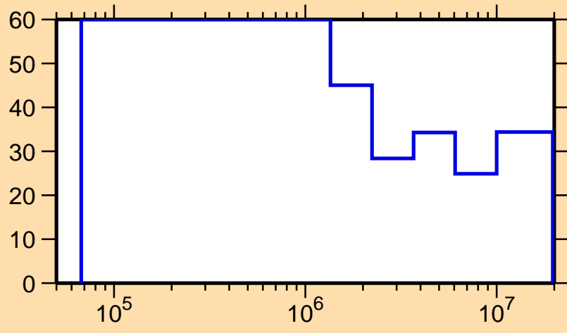
\Delta\sigma/\sigma vs. E for ^{187}\text{Au}(n,n\text{cont.})
