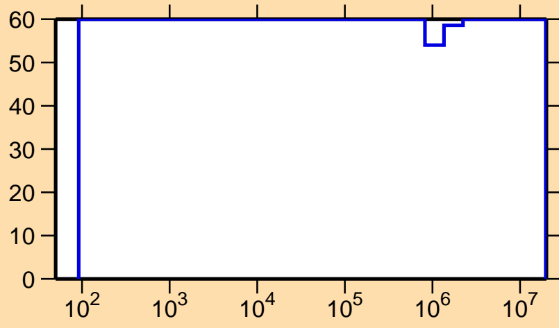
\Delta\sigma/\sigma vs. E for ^{187}\text{Au}(n,n_1)
