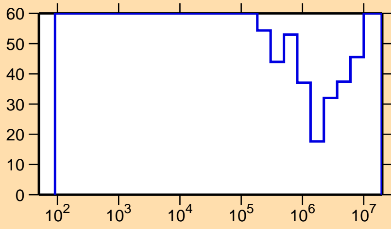
\Delta\sigma/\sigma vs. E for ^{187}\text{Au}(n,\gamma)
