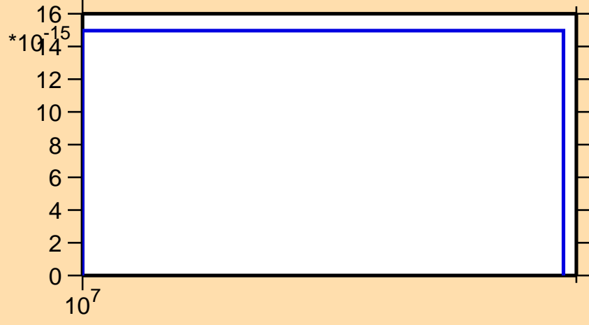
\sigma vs. E for ^{187}\text{Au} (mt 34)
