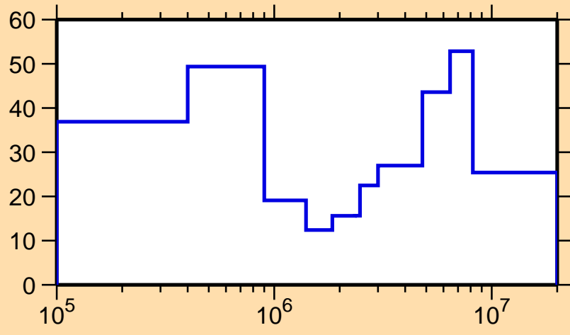
\Delta\sigma/\sigma vs. E for ^{187}\text{Au}(n, el.)
