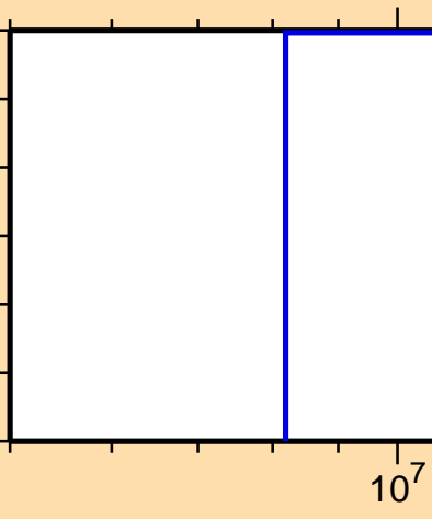
\sigma vs. E for ^{187}\text{Au}(n,3n\alpha)
