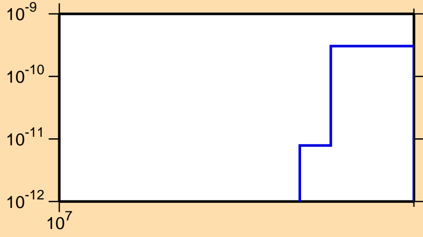
\sigma vs. E for ^{188}\text{Au}(\text{mt } 34)
