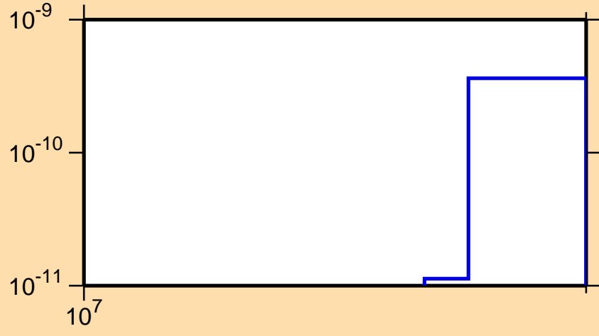
\sigma vs. E for ^{188}\text{Au}(n,pt)
