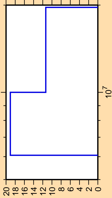
\Delta\sigma/\sigma vs. E for ^{188}\text{Au}(n,2n)
