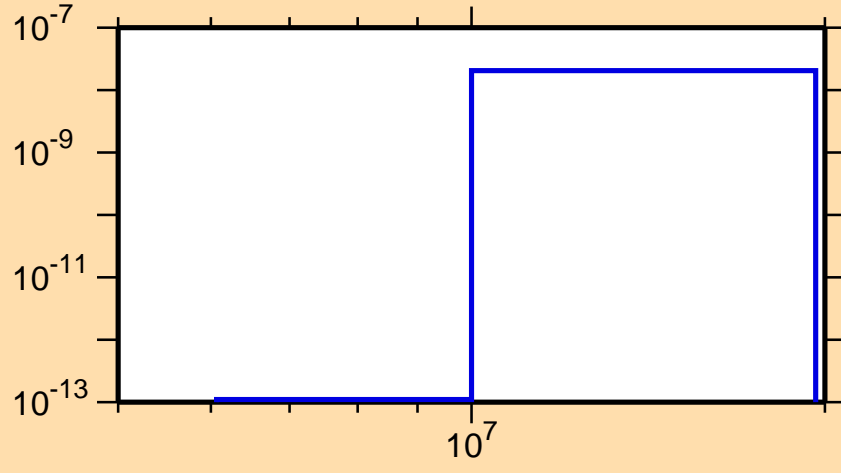
\sigma vs. E for ^{188}\text{Au}(\text{mt117})
