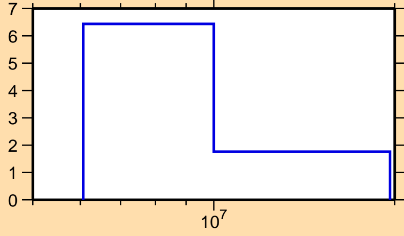
\Delta\sigma/\sigma vs. E for ^{188}\text{Au}(n,\text{tot.})
