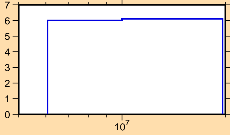
\Delta\sigma/\sigma vs. E for ^{188}\text{Au}(n,\text{nonel.})
