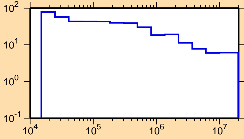
\Delta\sigma/\sigma vs. E for ^{188}\text{Au}(n,\text{nonel.})
