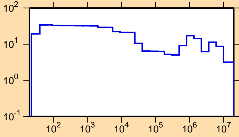
\Delta\sigma/\sigma vs. E for ^{188}\text{Au}(n,\text{el.})
