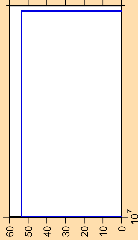
\Delta\sigma/\sigma vs. E for ^{188}\text{Au}(n,\text{pd})
