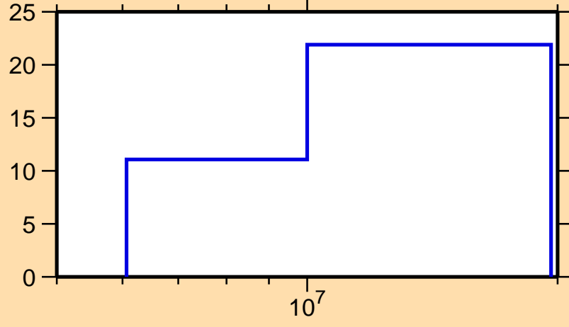
\Delta\sigma/\sigma vs. E for ^{188}\text{Au}(n,\text{inel.})
