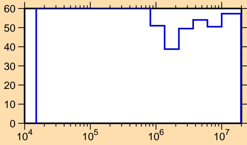
\Delta\sigma/\sigma vs. E for ^{188}\text{Au}(n,n_1)
