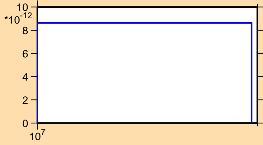
\sigma vs. E for ^{188}\text{Au}(n,\text{pd})
