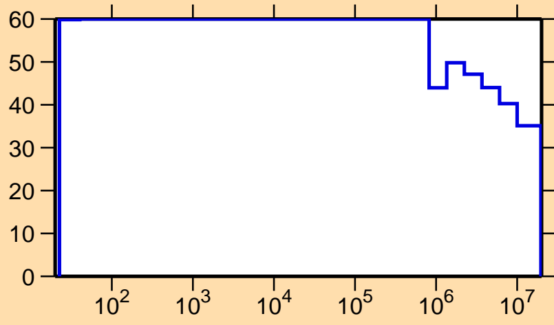
\Delta\sigma/\sigma vs. E for ^{188}\text{Au}(n,p)
