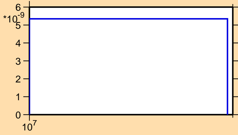
\sigma vs. E for ^{188}\text{Au}(n,nt)
