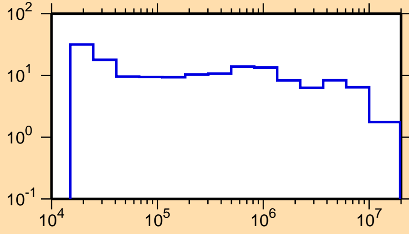
\Delta\sigma/\sigma vs. E for ^{188}\text{Au}(n,\text{tot.})
