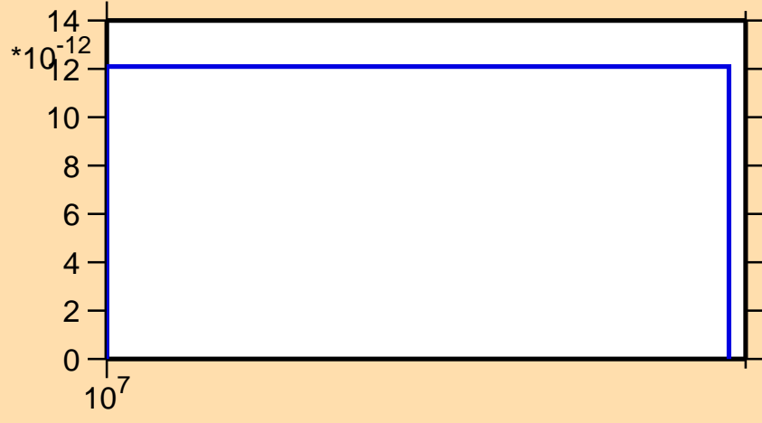
\sigma vs. E for ^{188}\text{Au}(n,3n\alpha)
