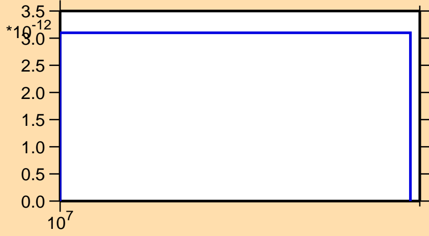
\sigma vs. E for ^{188}\text{Au}(\text{mt } 34)
