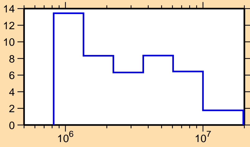
\Delta\sigma/\sigma vs. E for ^{188}\text{Au}(n, \text{tot.})
