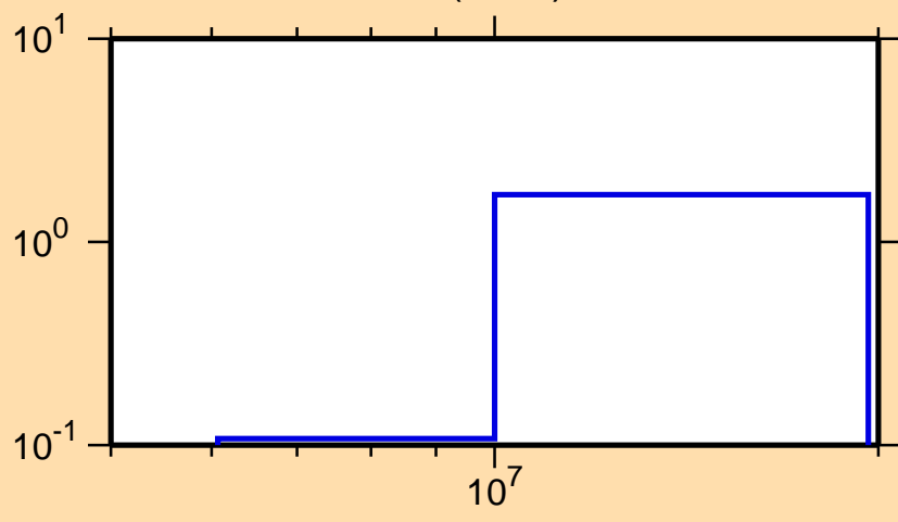
\sigma vs. E for ^{188}\text{Au}(n,2n)
