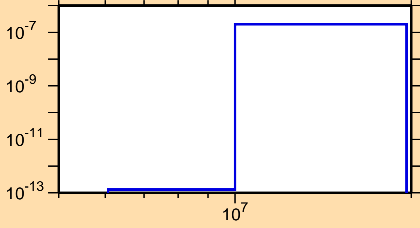
\sigma vs. E for ^{188}\text{Au}(n,\text{He3})
