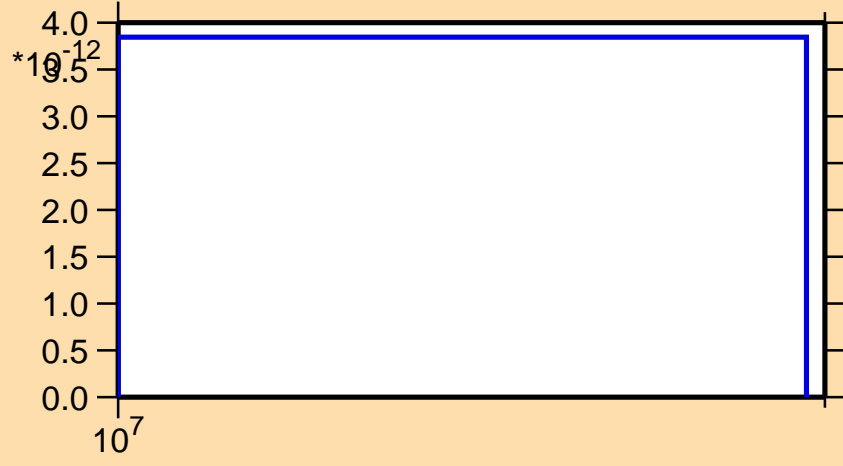
\sigma vs. E for ^{188}\text{Au}(n,\text{pt})
