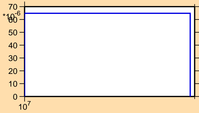
\sigma vs. E for ^{188}\text{Au}(n,3n)
