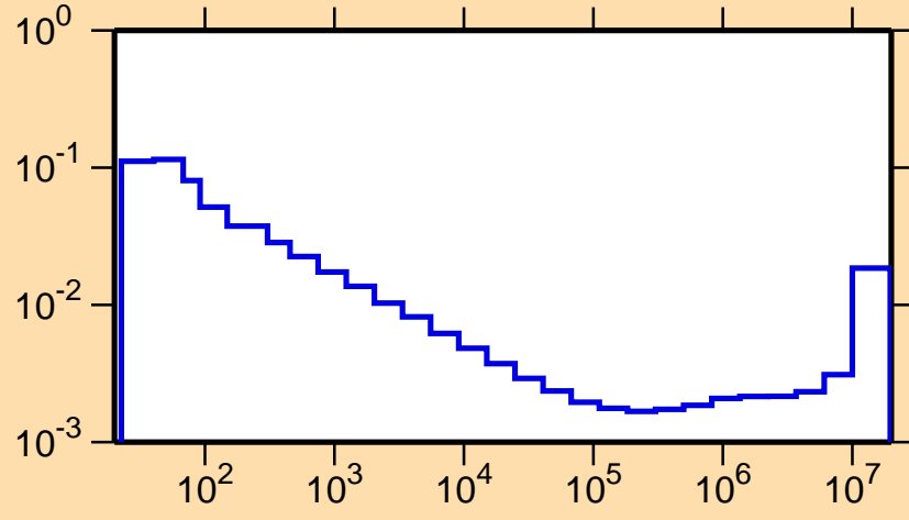
\sigma vs. E for ^{188}\text{Au}(n,\alpha)
