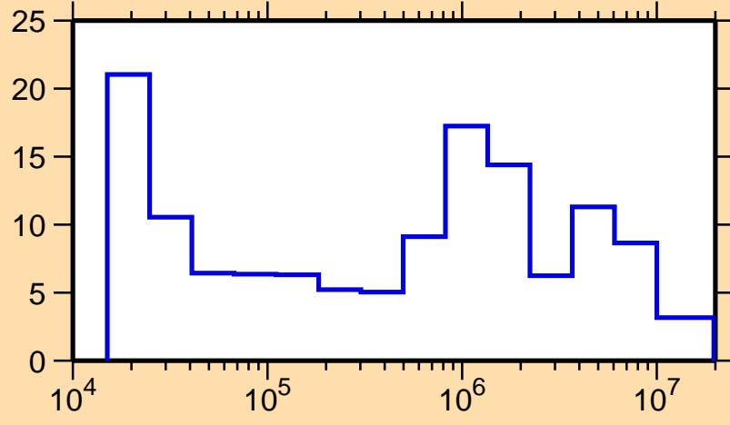
\Delta\sigma/\sigma vs. E for ^{188}\text{Au}(n,\text{el.})
