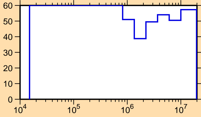
\Delta\sigma/\sigma vs. E for ^{188}\text{Au}(n,n_1)
