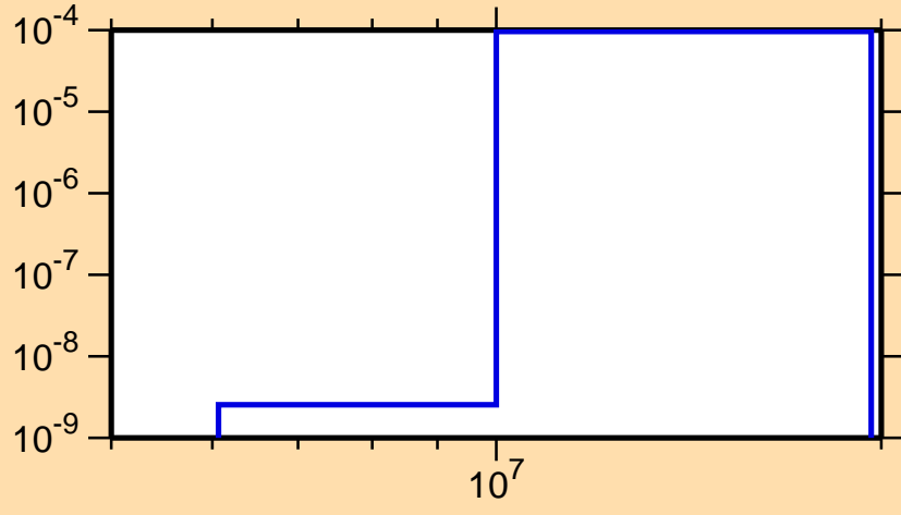
\sigma vs. E for ^{188}\text{Au}(n,2n\alpha)
