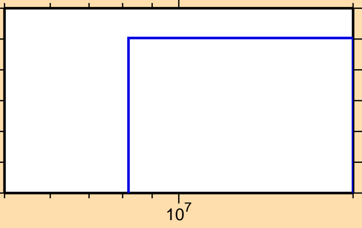
\sigma vs. E for ^{188}\text{Au}(n,nt)
