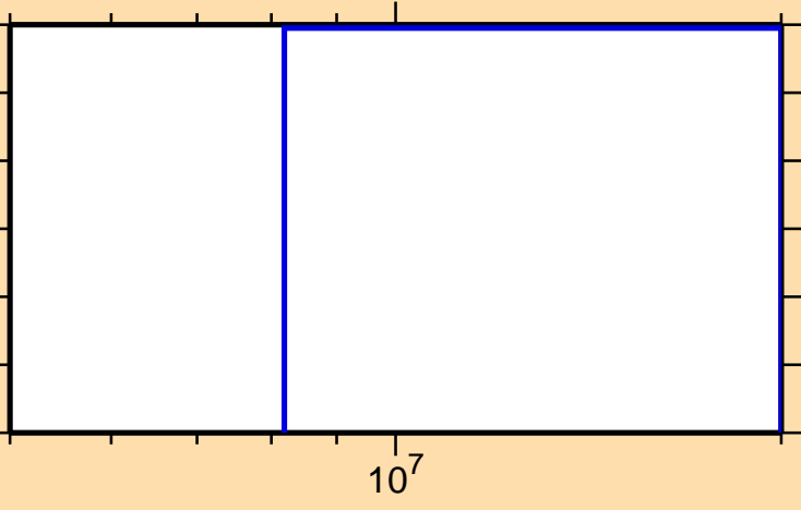
\sigma vs. E for ^{188}\text{Au}(n,2np)
