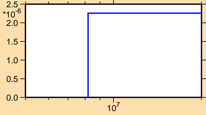
\sigma vs. E for ^{188}\text{Au}(n,nd)
