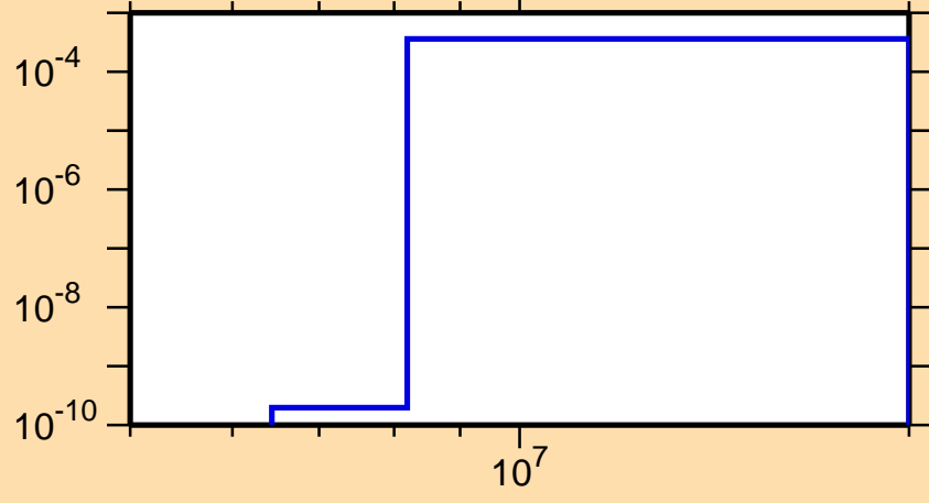
\sigma vs. E for ^{188}\text{Au}(n,t)
