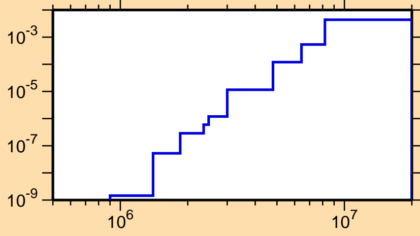
\sigma vs. E for ^{188}\text{Au}(n,n\alpha)
